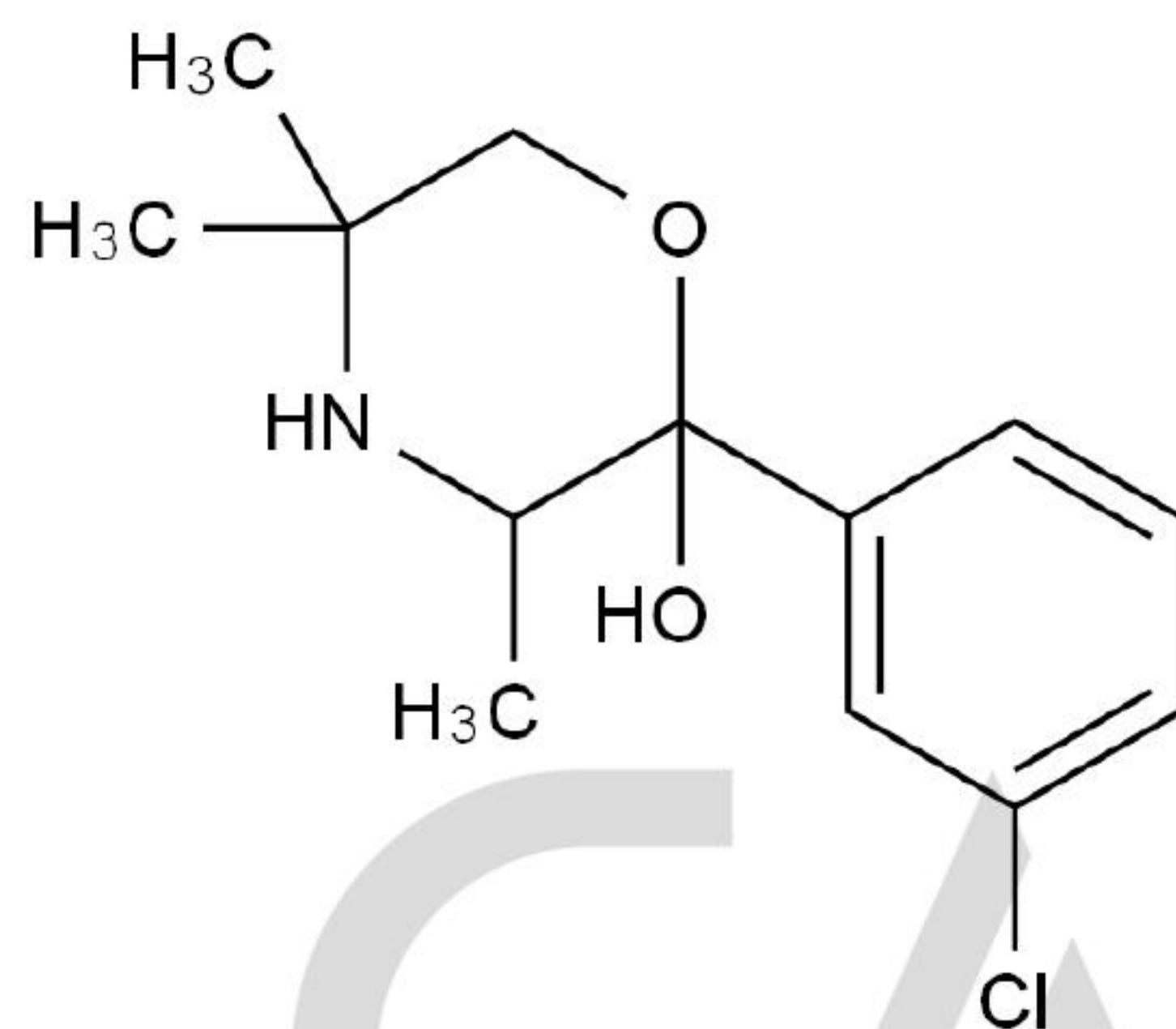
Chemical Structure:
