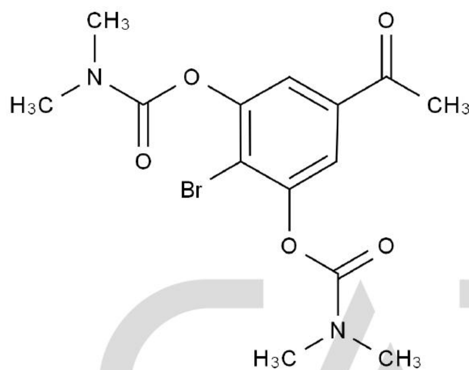
Chemical Structure:
