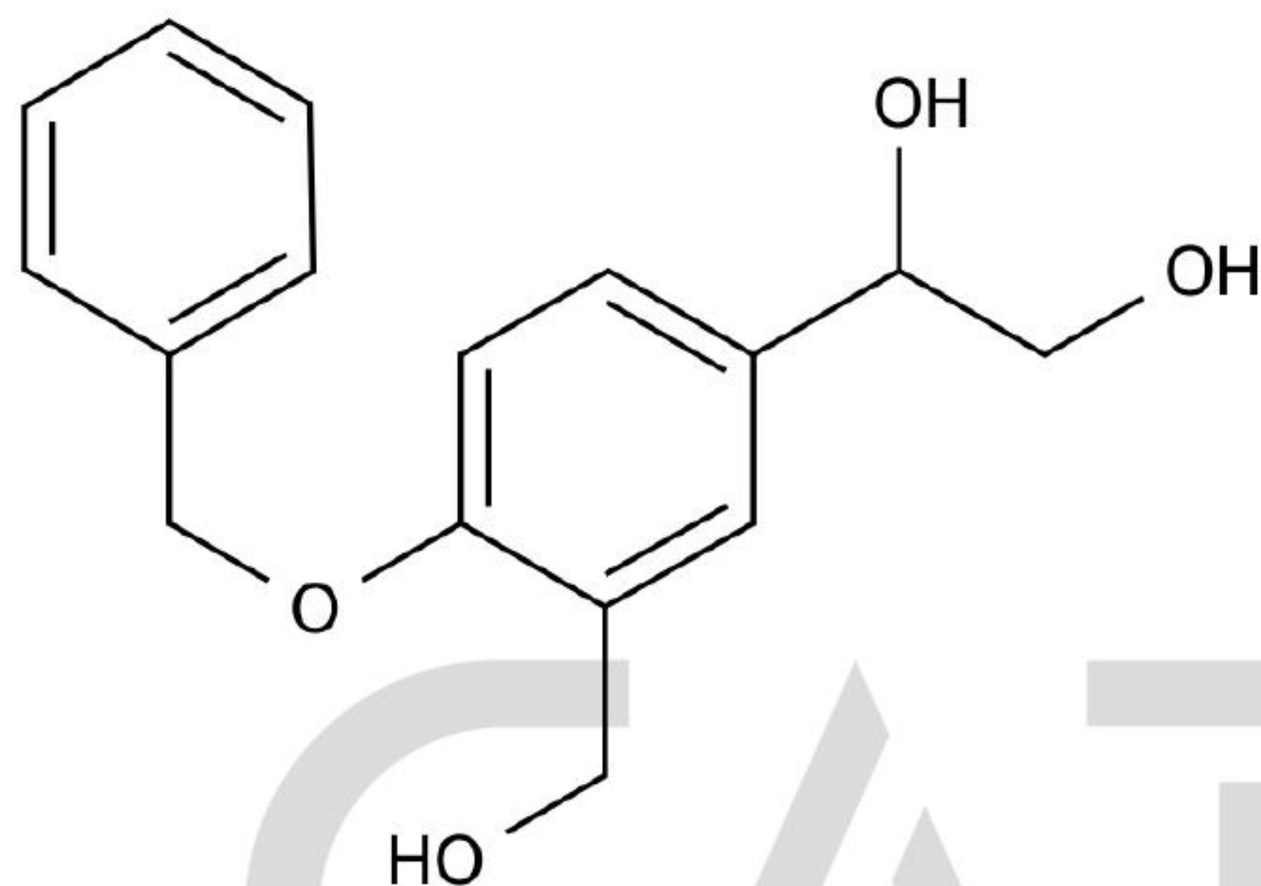
Chemical Structure:
