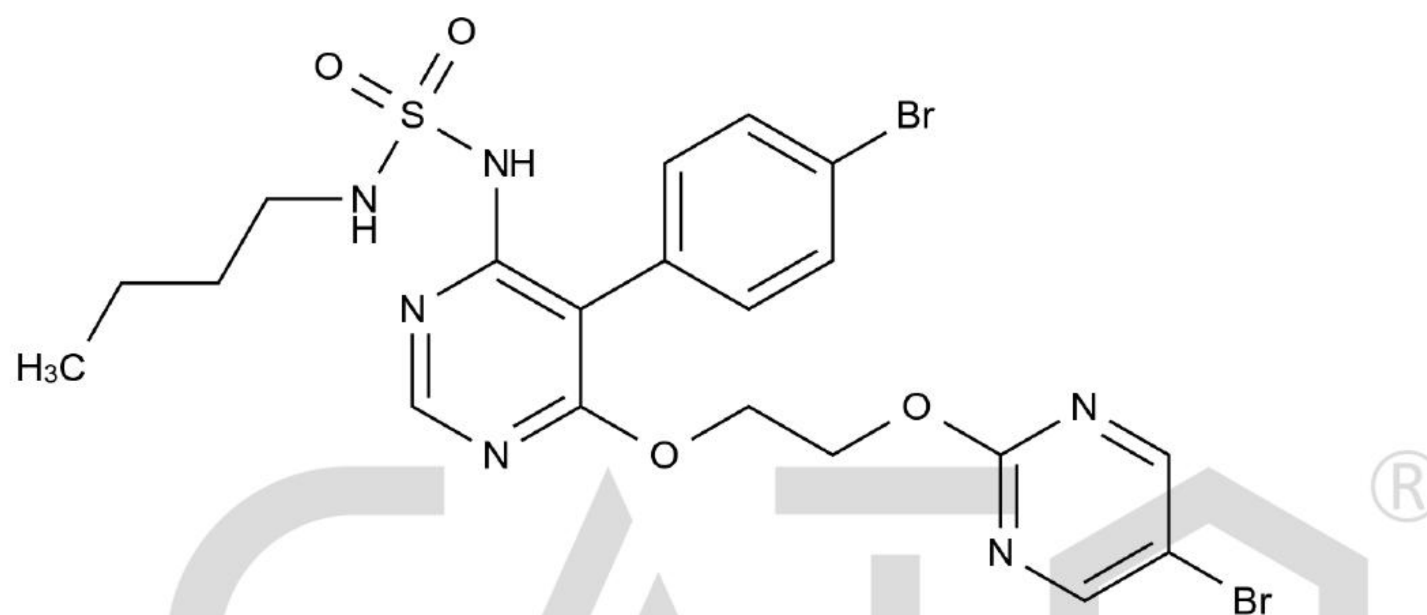
Chemical Structure:
