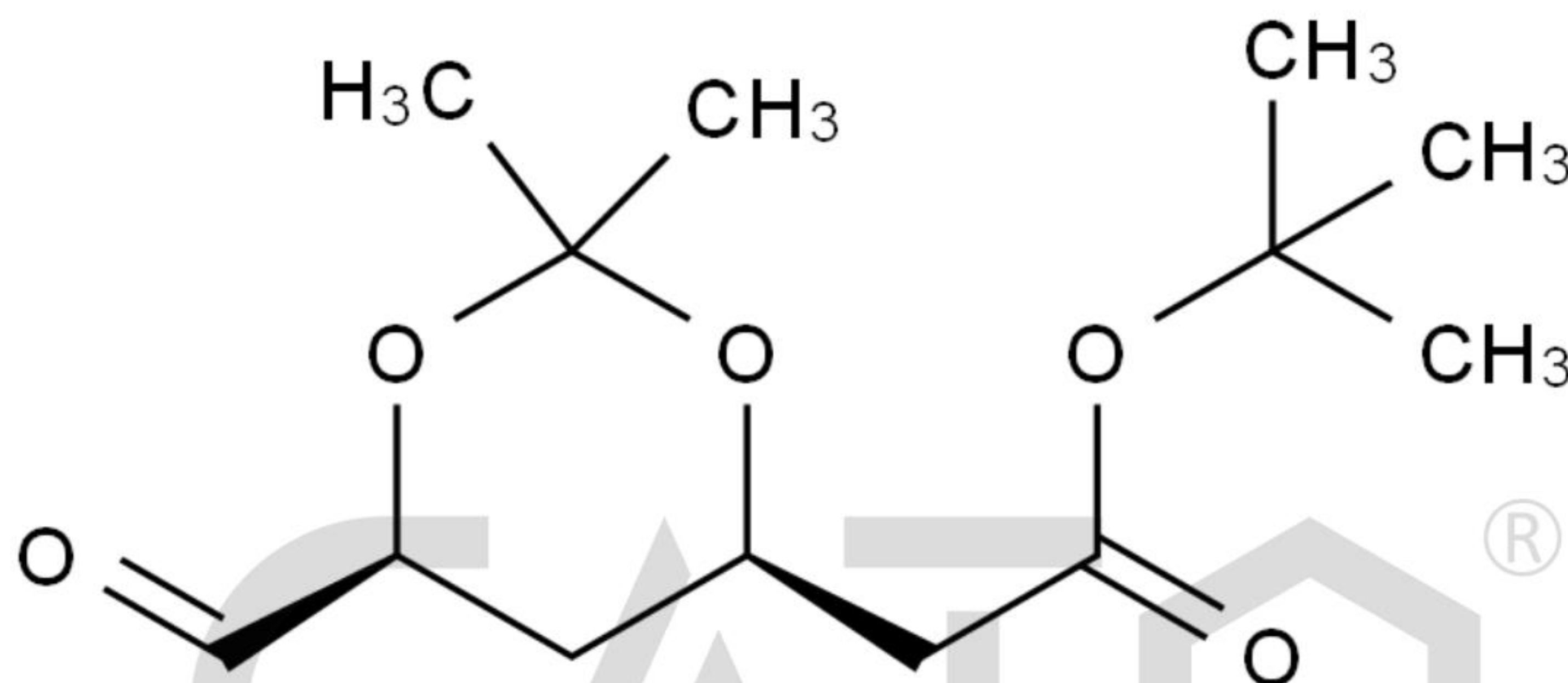
Chemical Structure:
