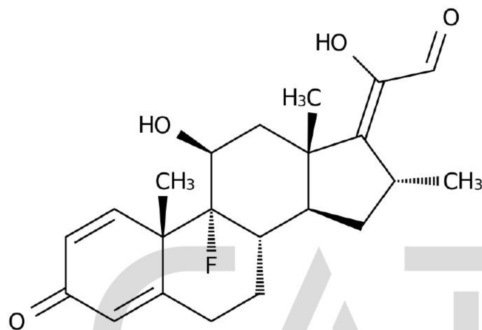
Chemical Structure:
