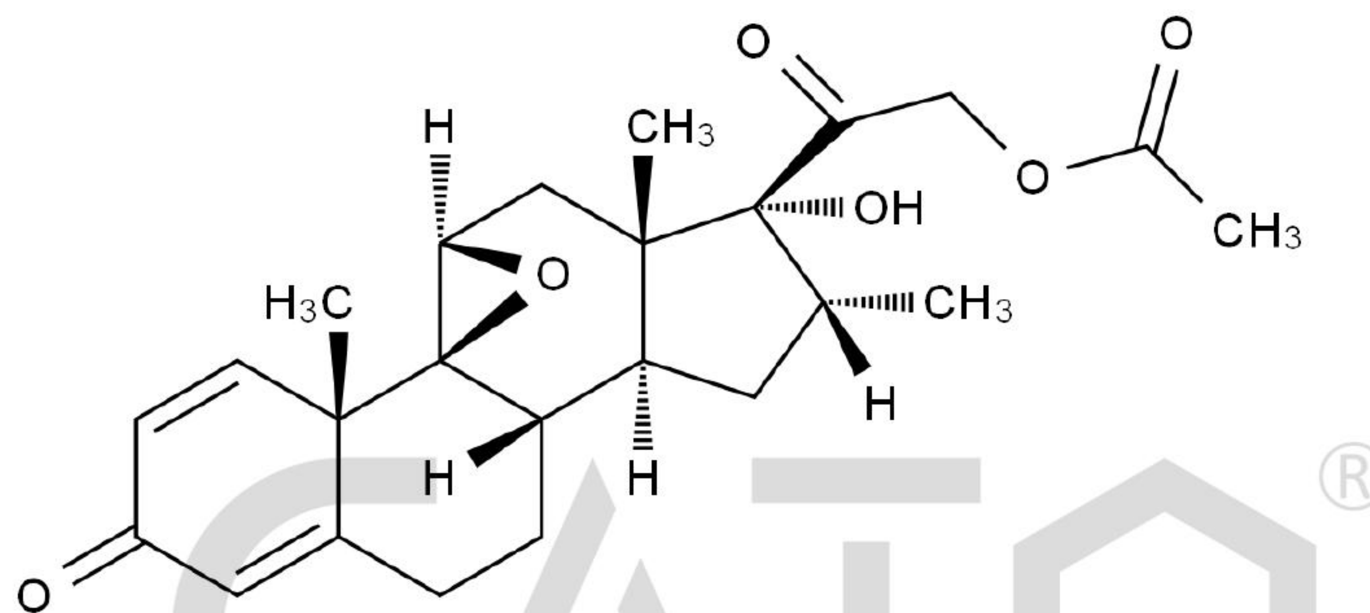
Chemical Structure:
