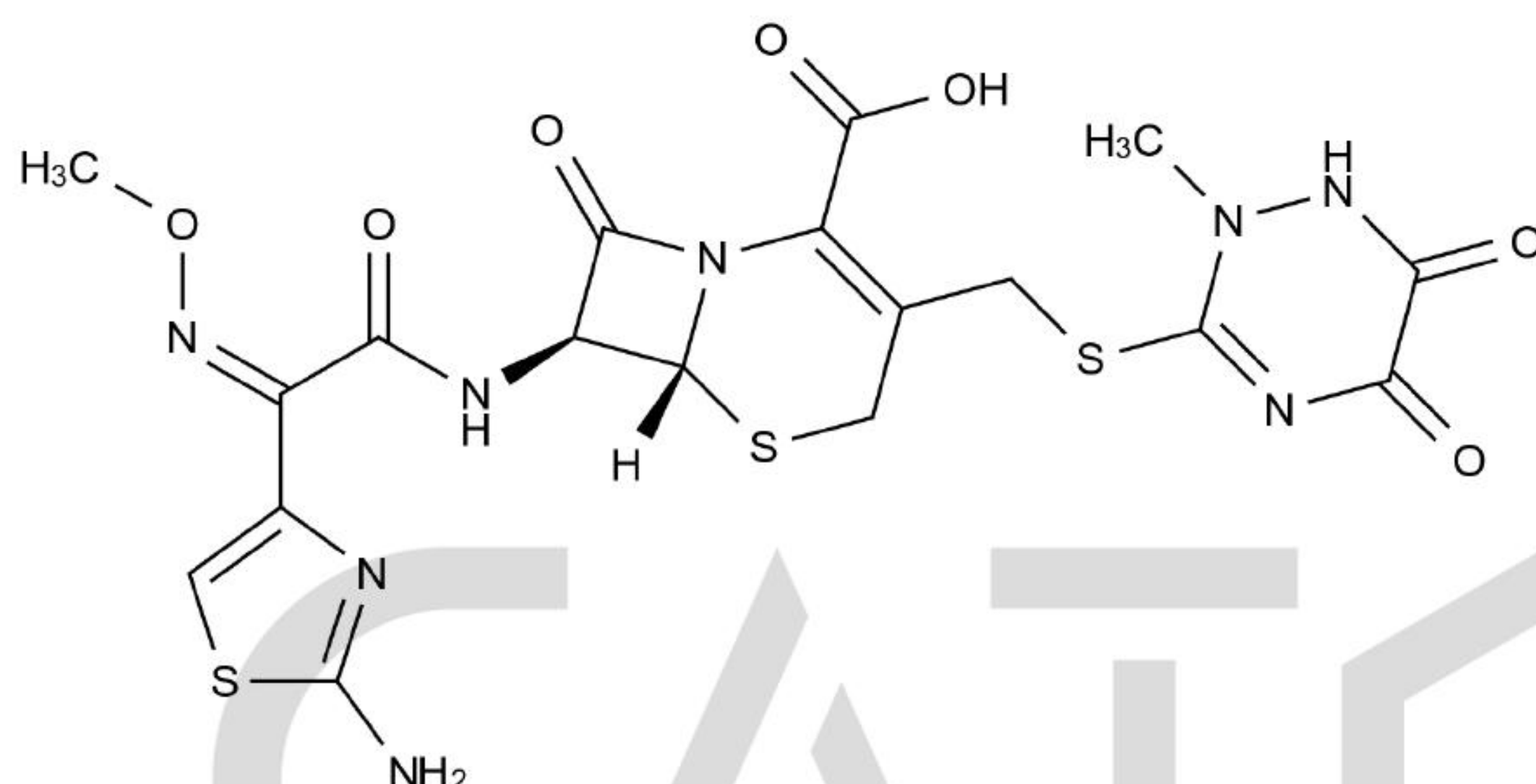
Chemical Structure:
