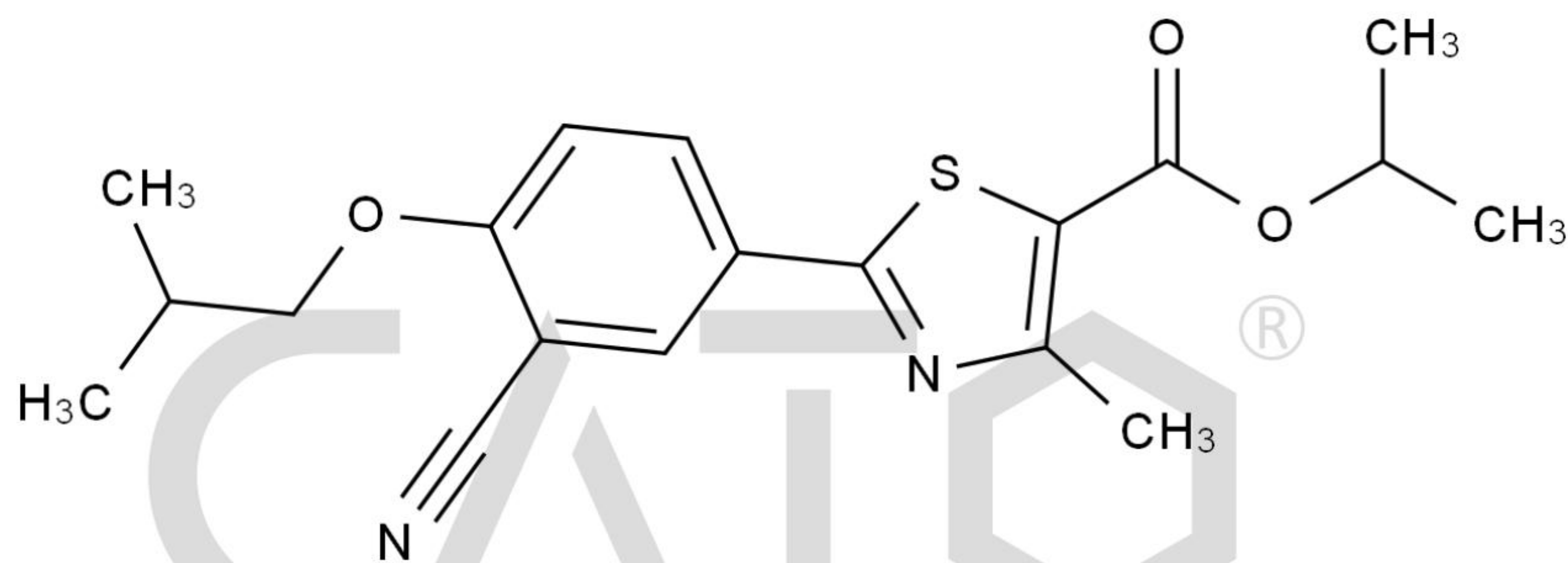
Chemical Structure:
