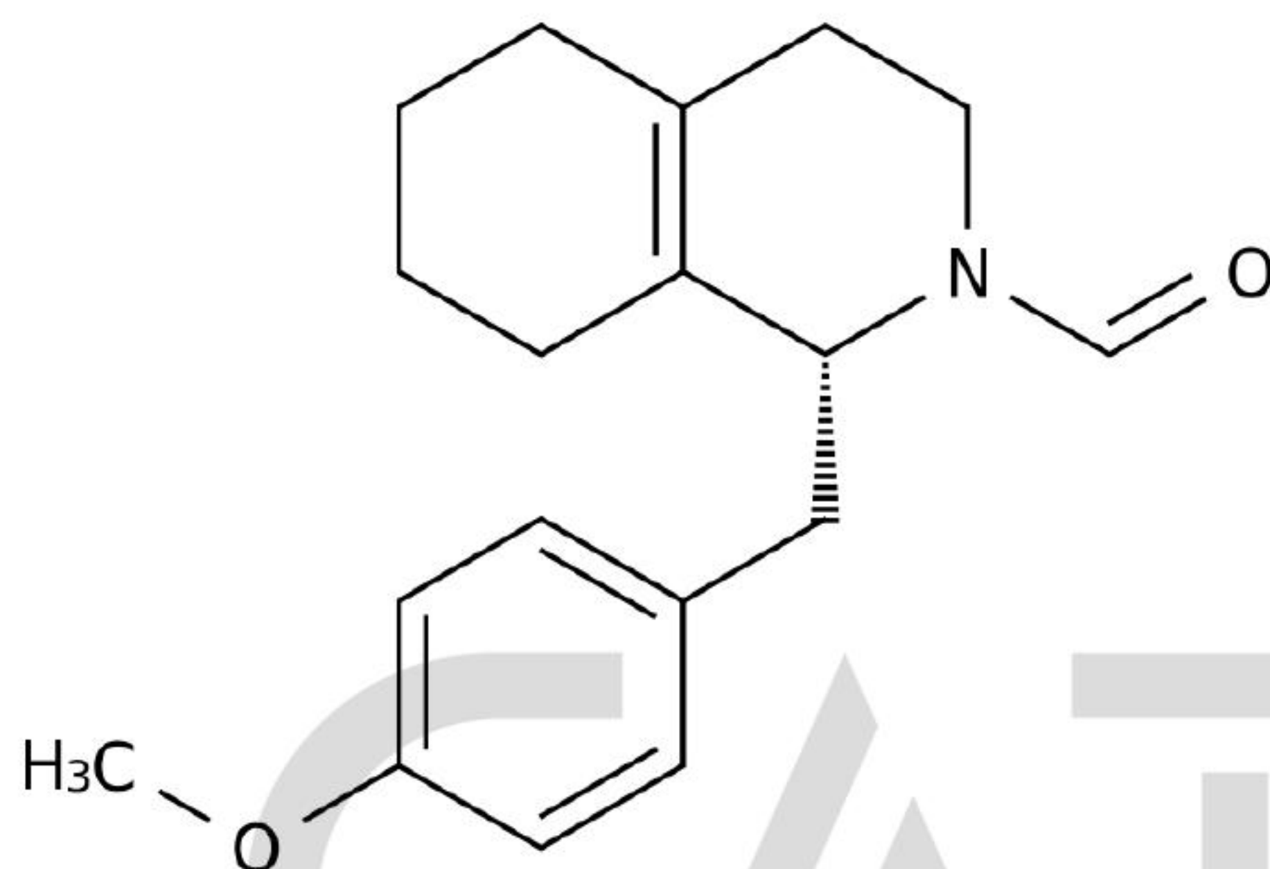
Chemical Structure:
