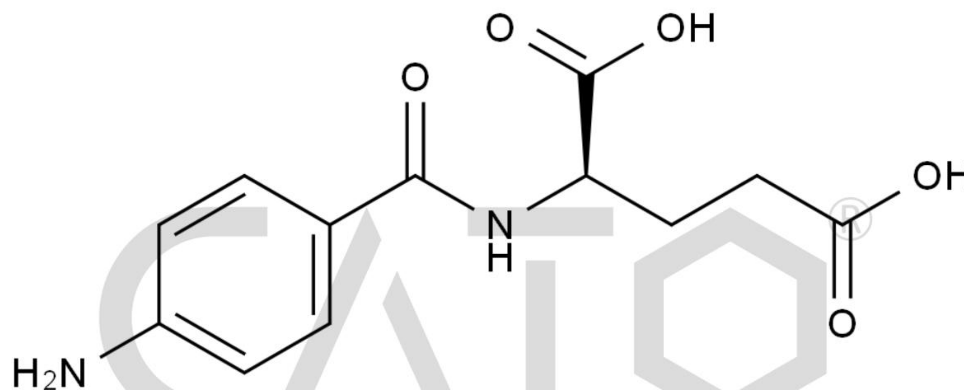
Chemical Structure:
