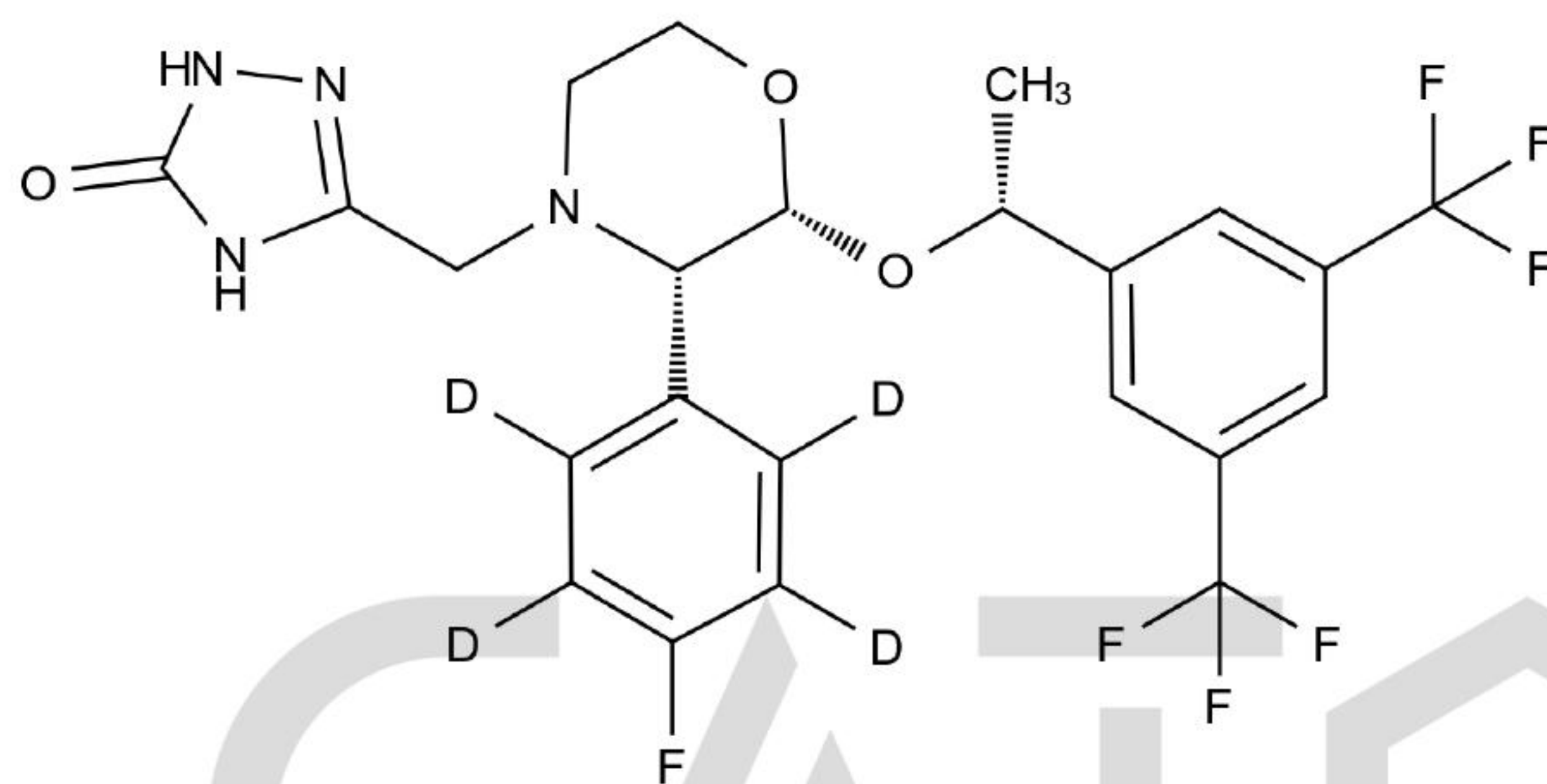
Chemical Structure:
