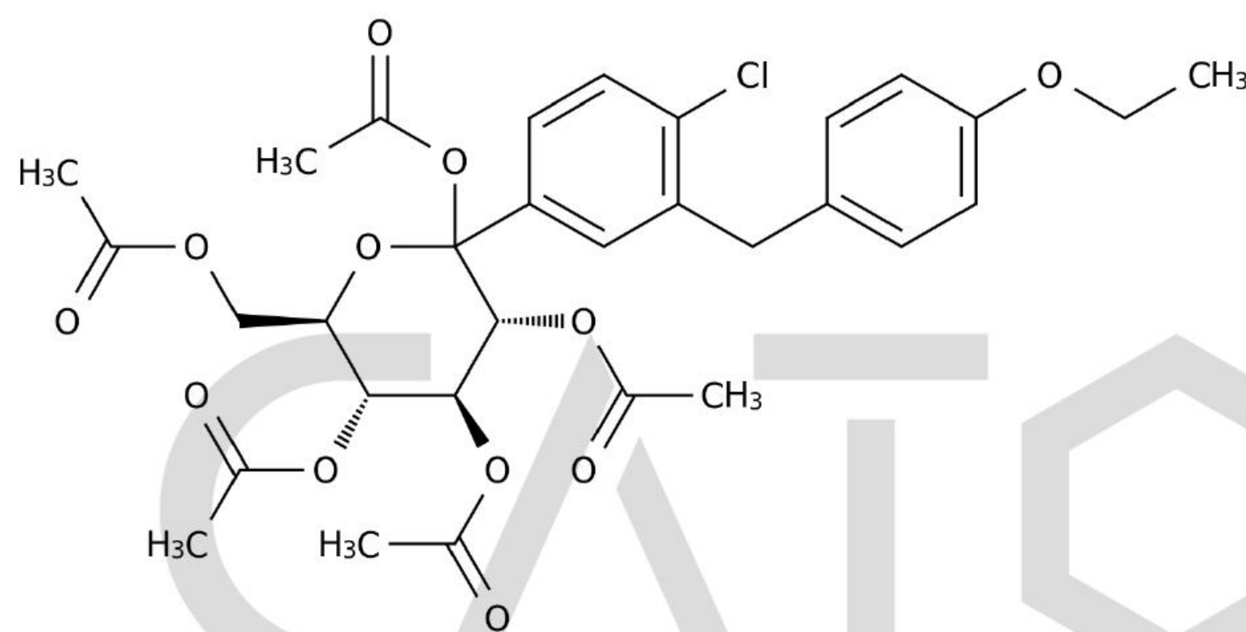
Chemical Structure:
