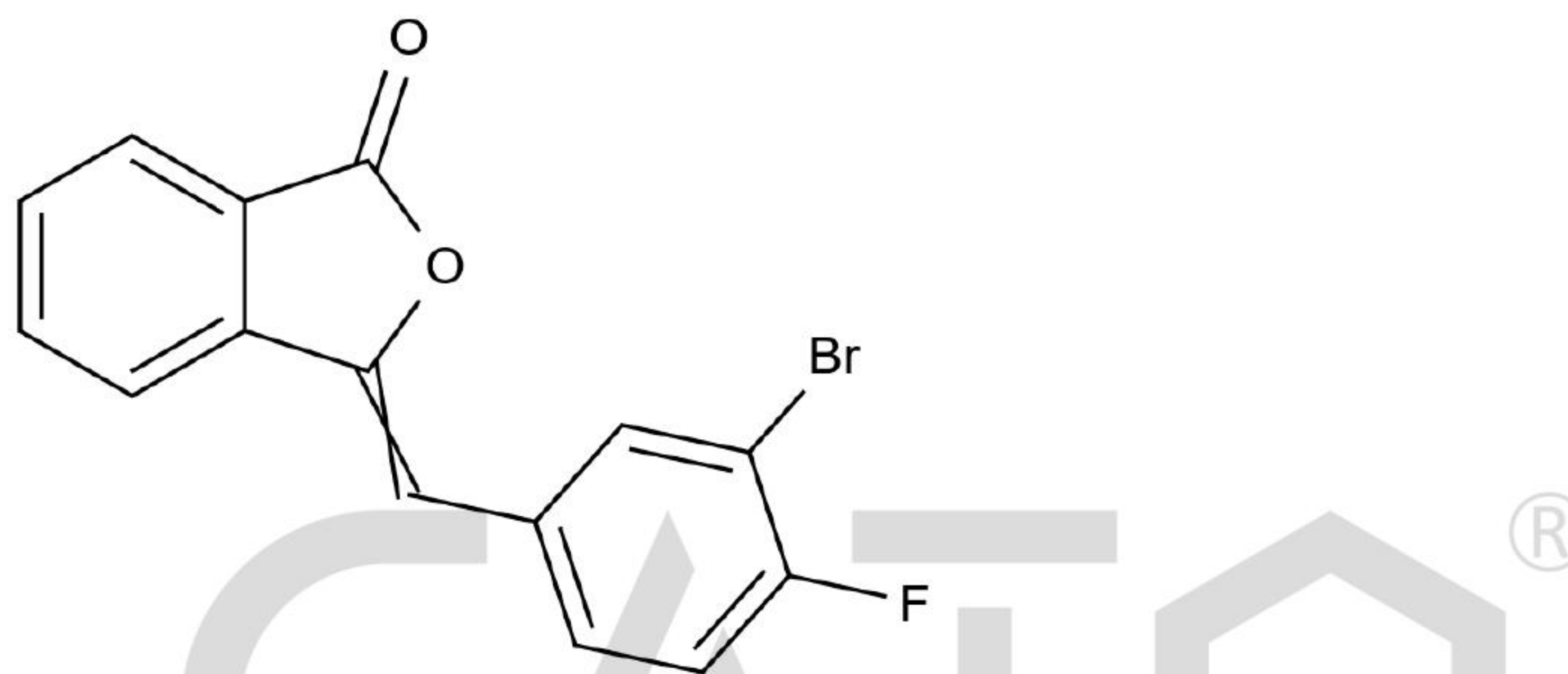
Chemical Structure:
