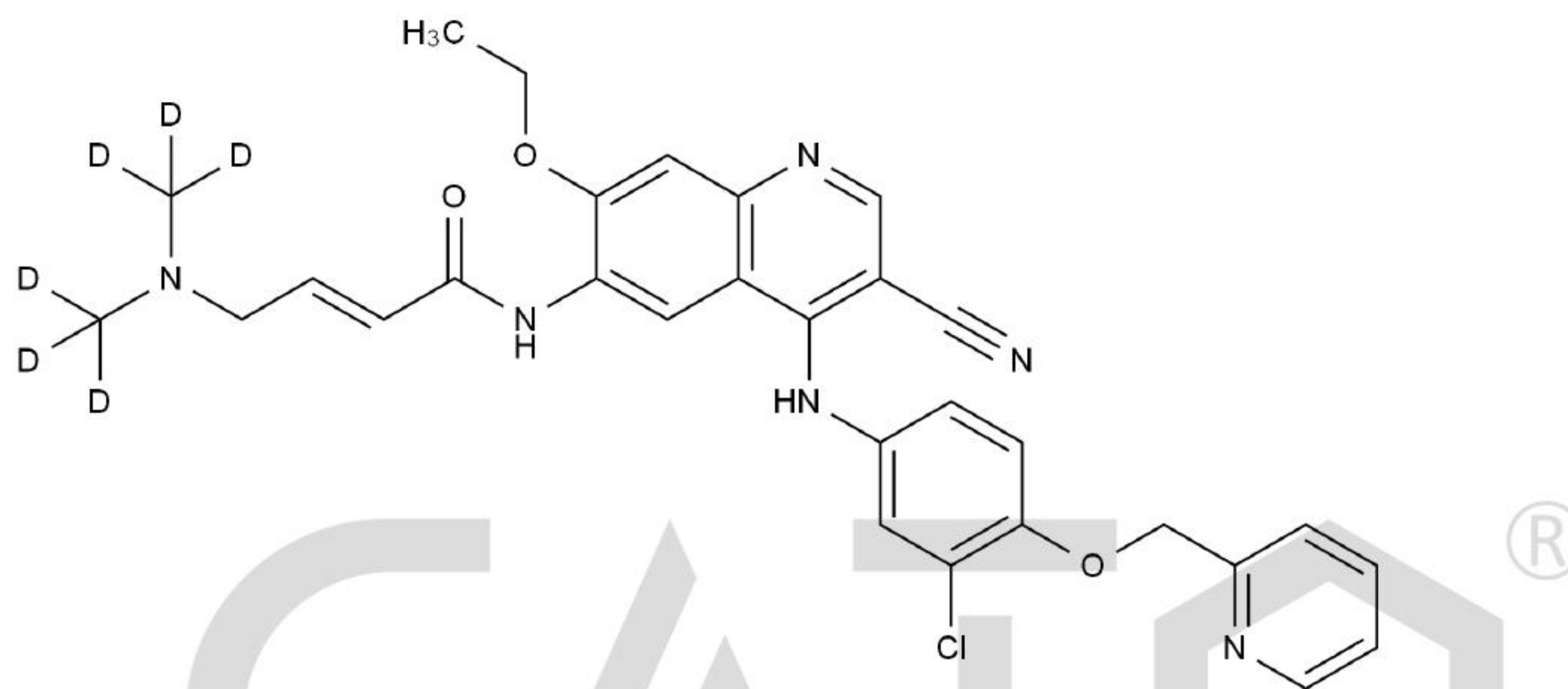
Chemical Structure:
