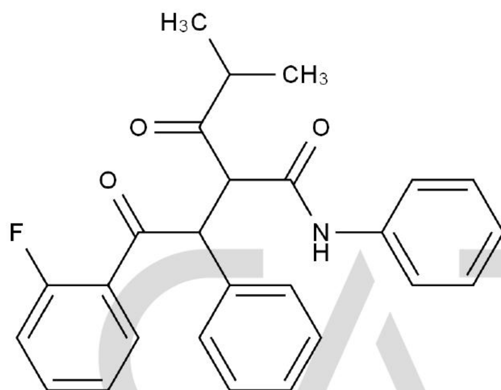
Chemical Structure:
