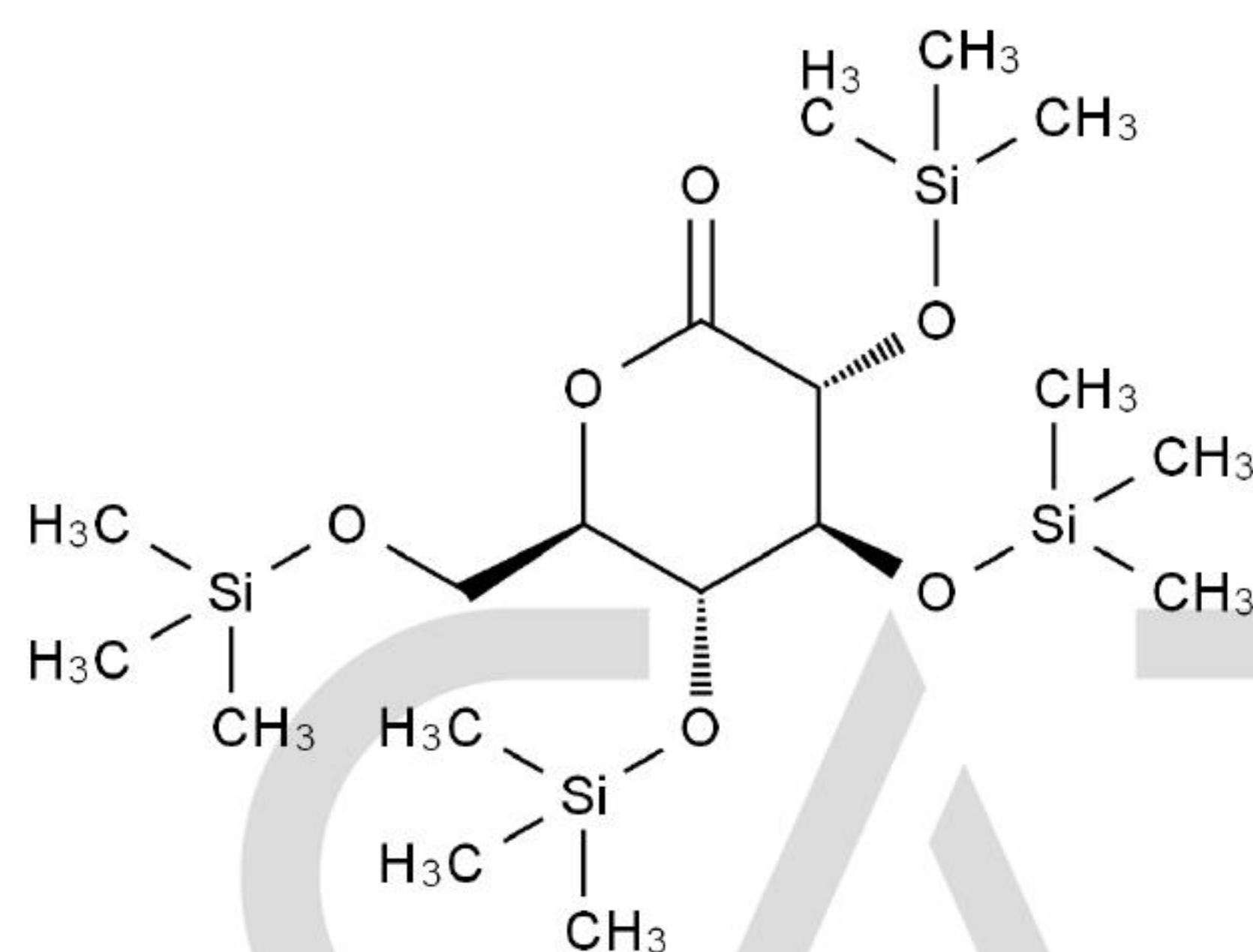
Chemical Structure:
