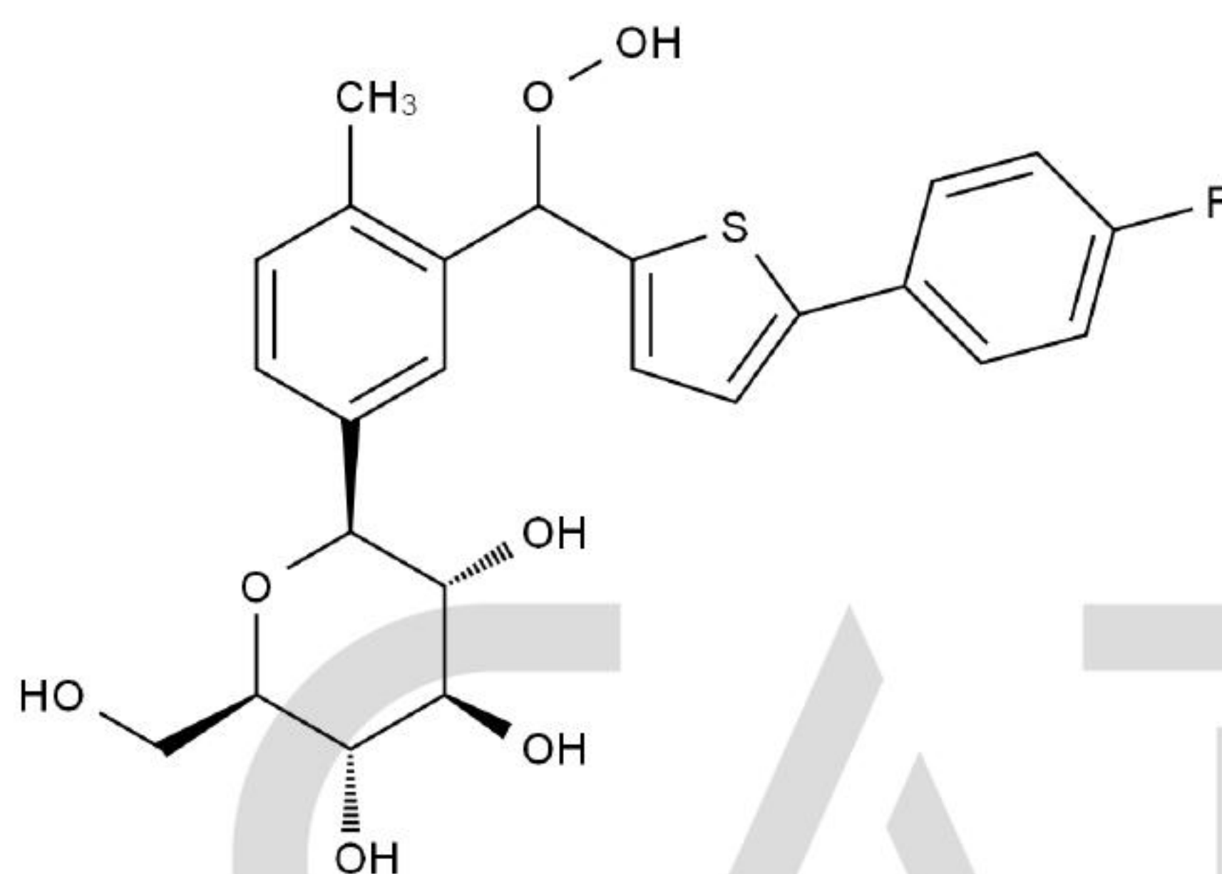
Chemical Structure:
