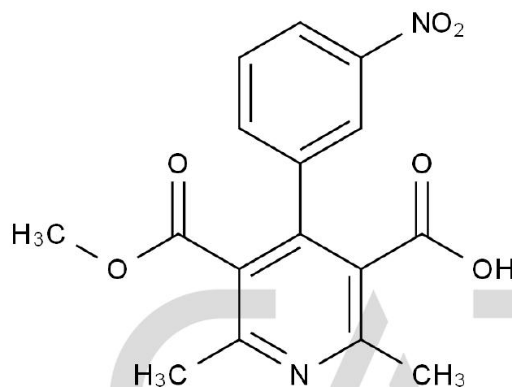
Chemical Structure:
