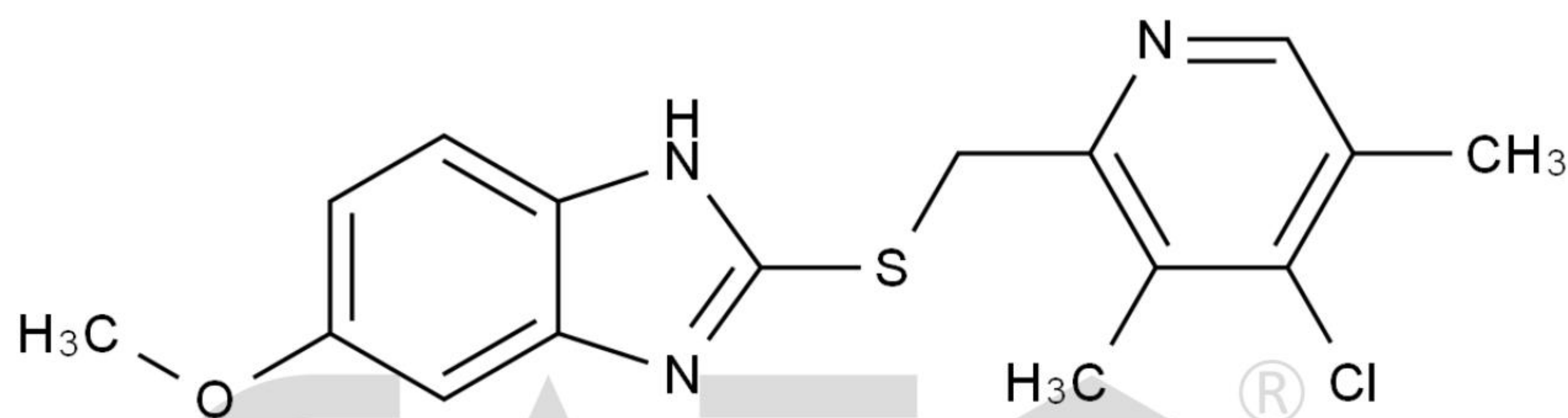
Chemical Structure:
