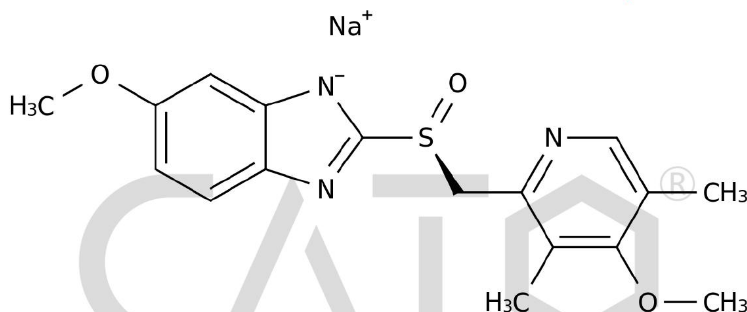
Chemical Structure:
