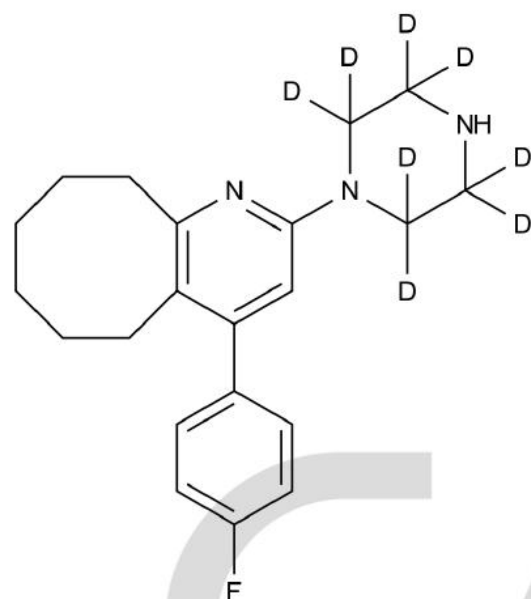
Chemical Structure:
