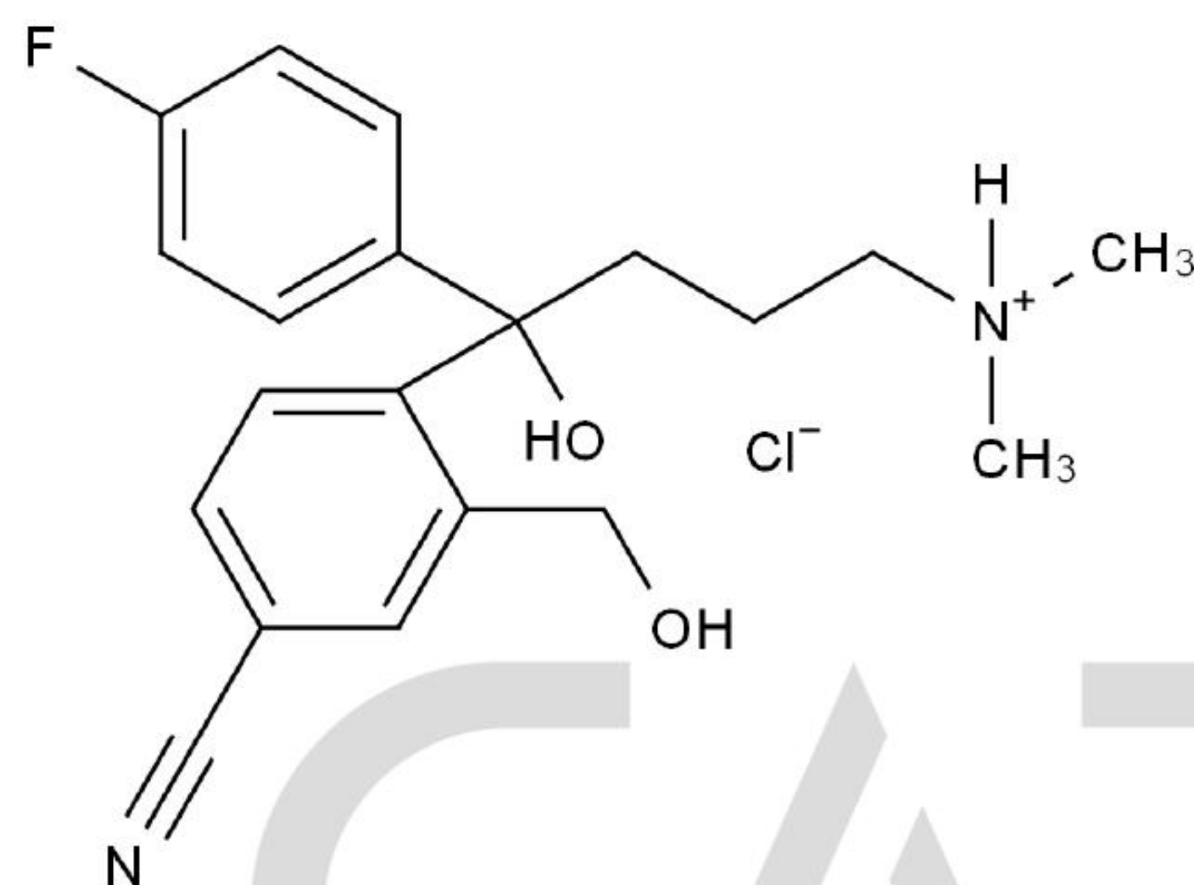
Chemical Structure:
