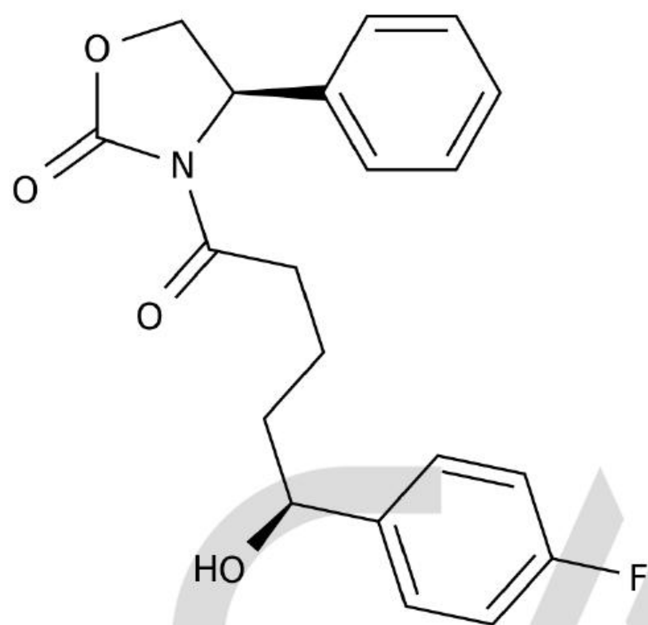
Chemical Structure:
