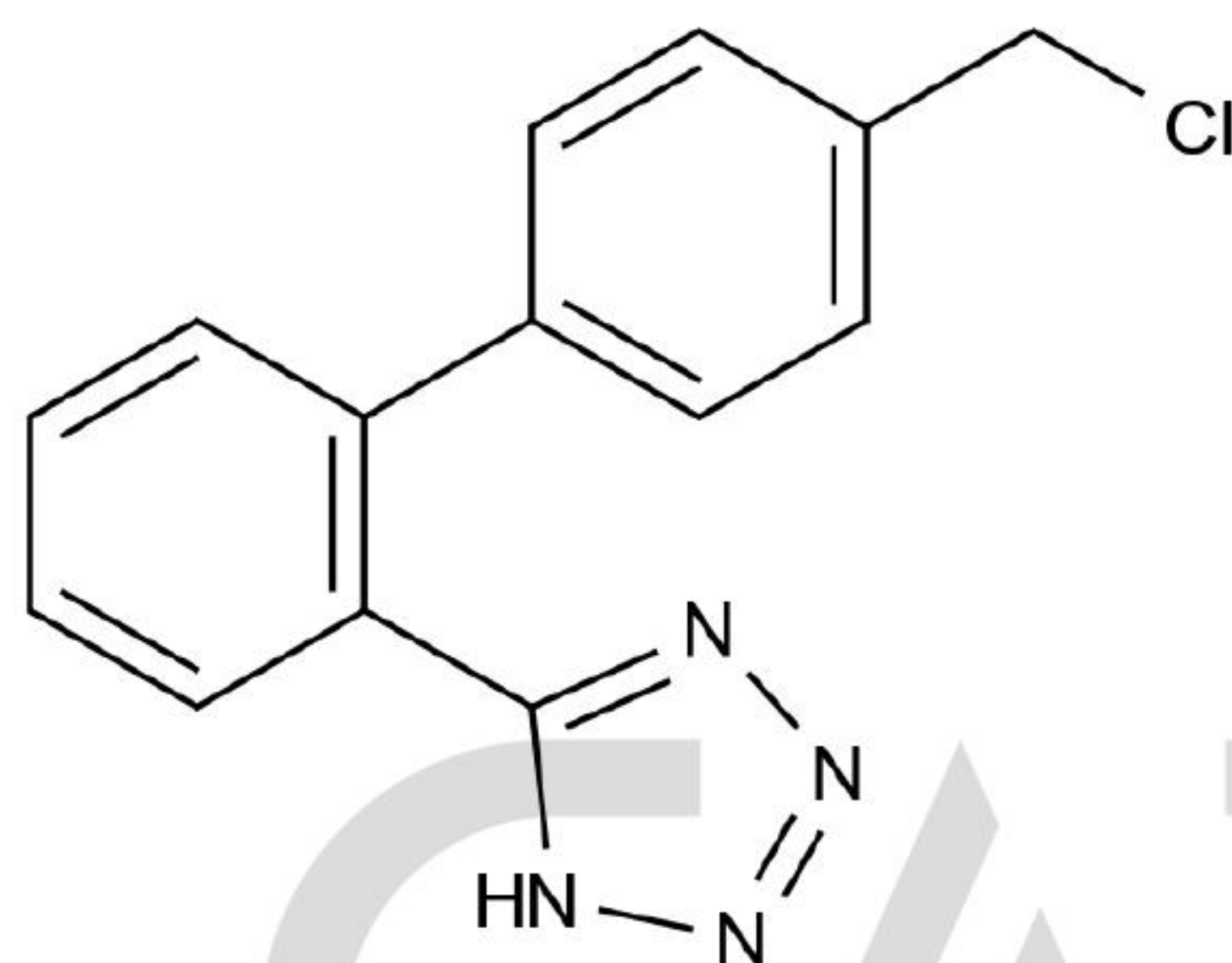
Chemical Structure:
