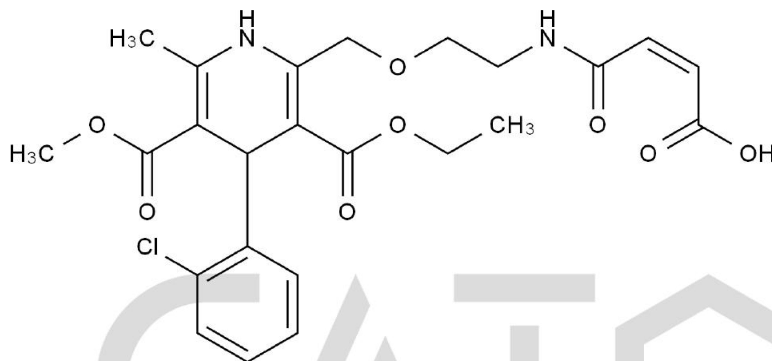
Chemical Structure:
