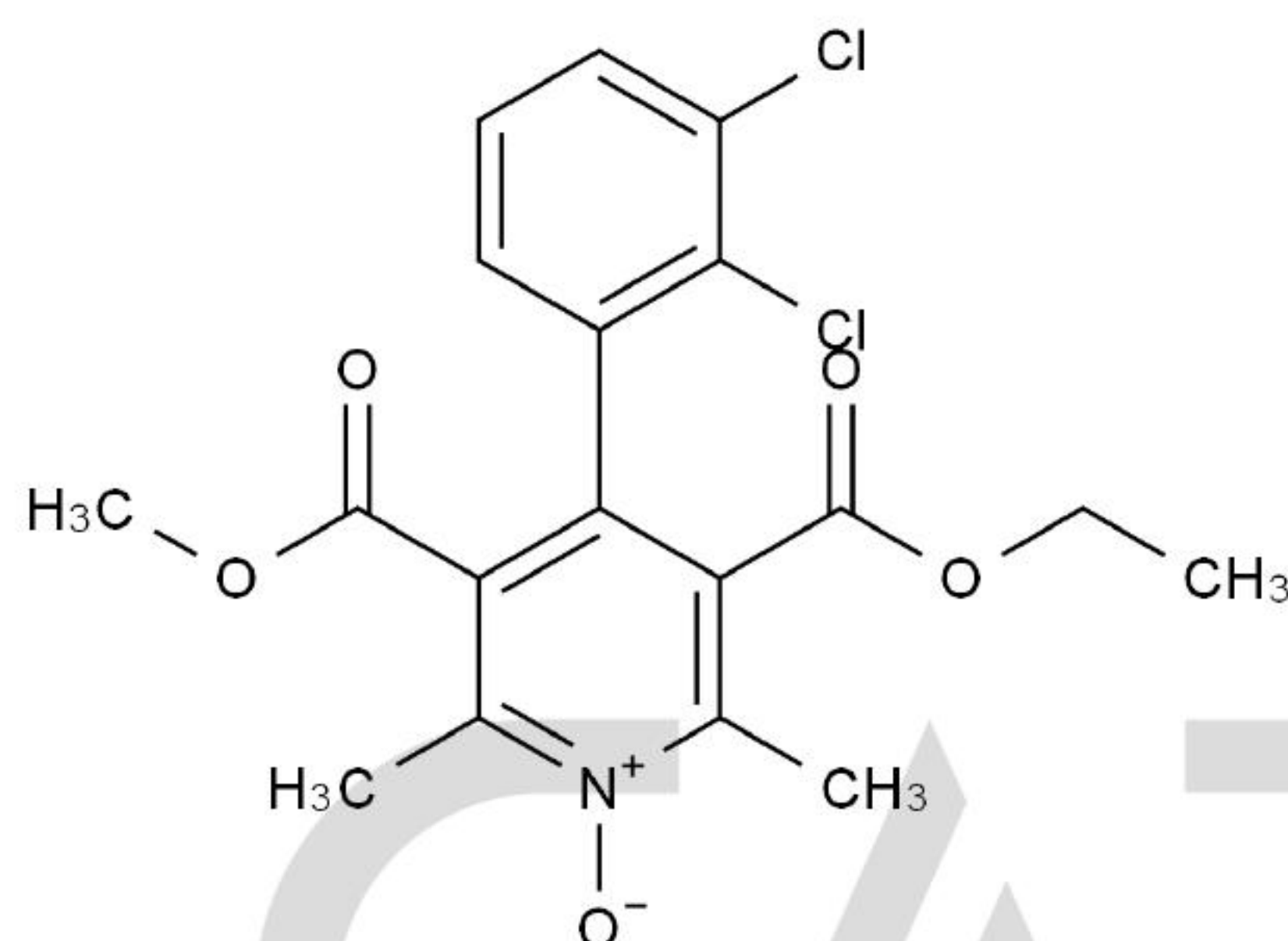
Chemical Structure:
