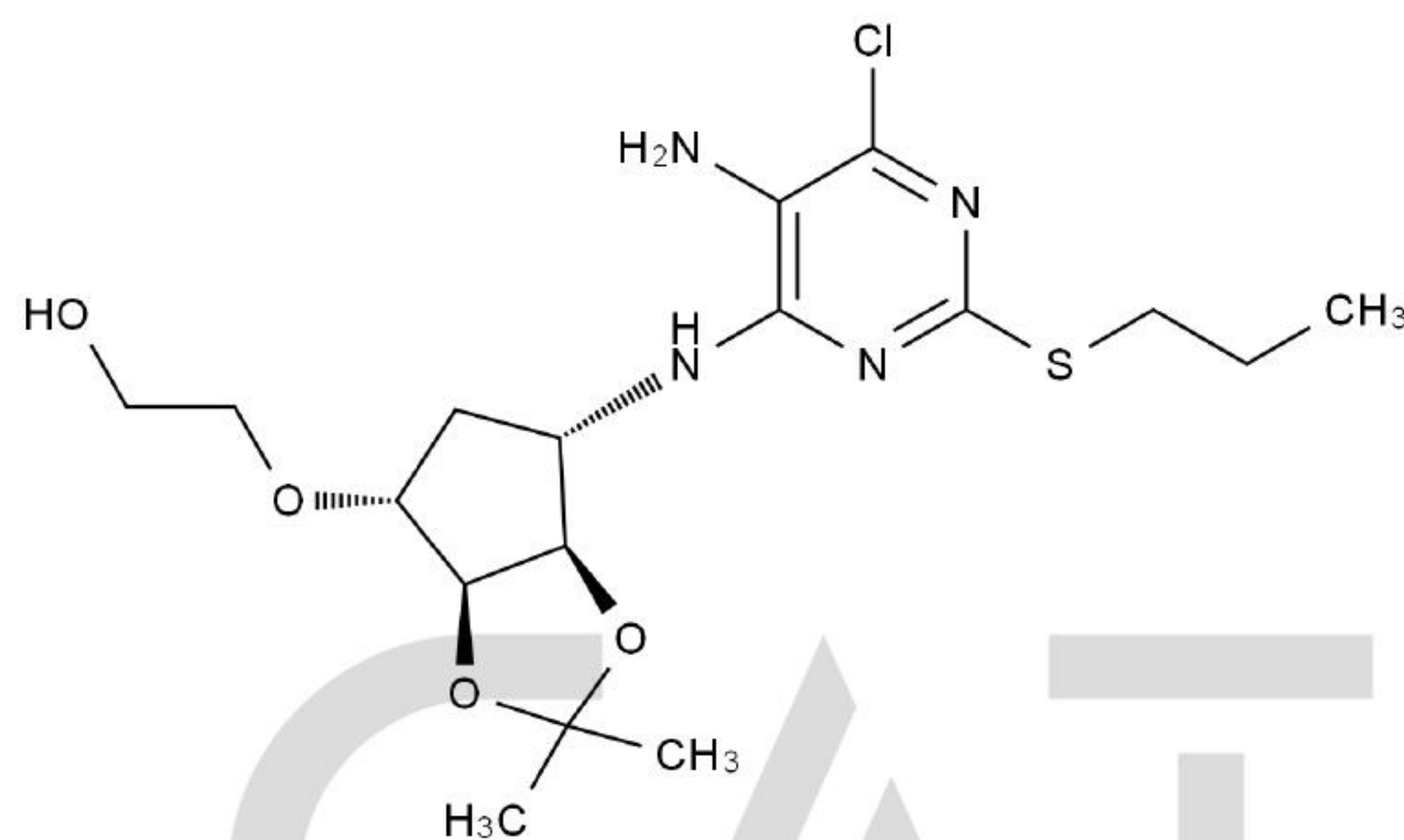
Chemical Structure:
