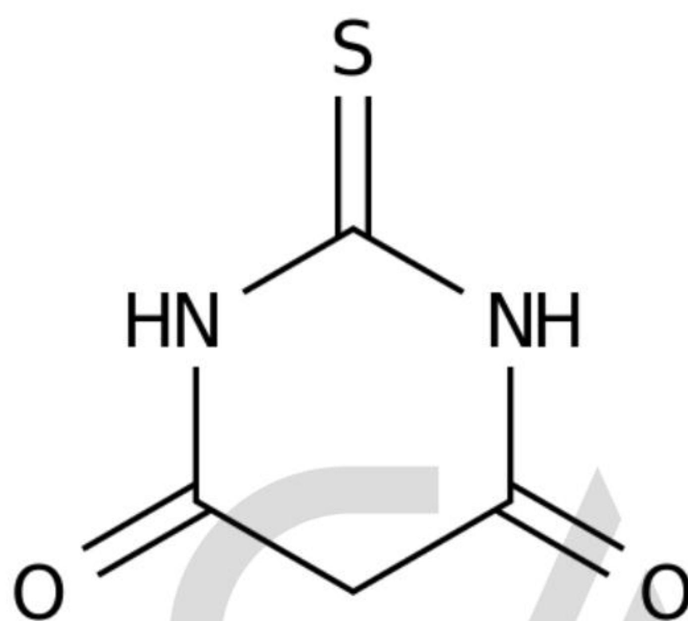
Chemical Structure:
