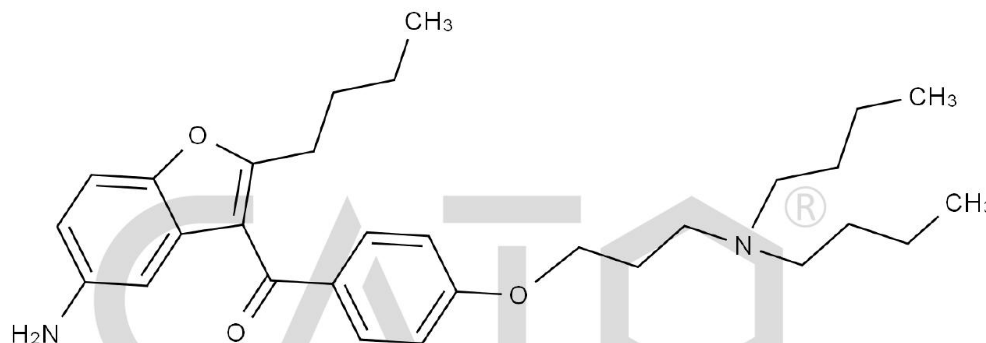
Chemical Structure:
