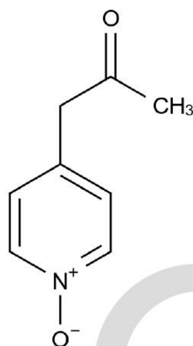
Chemical Structure:
