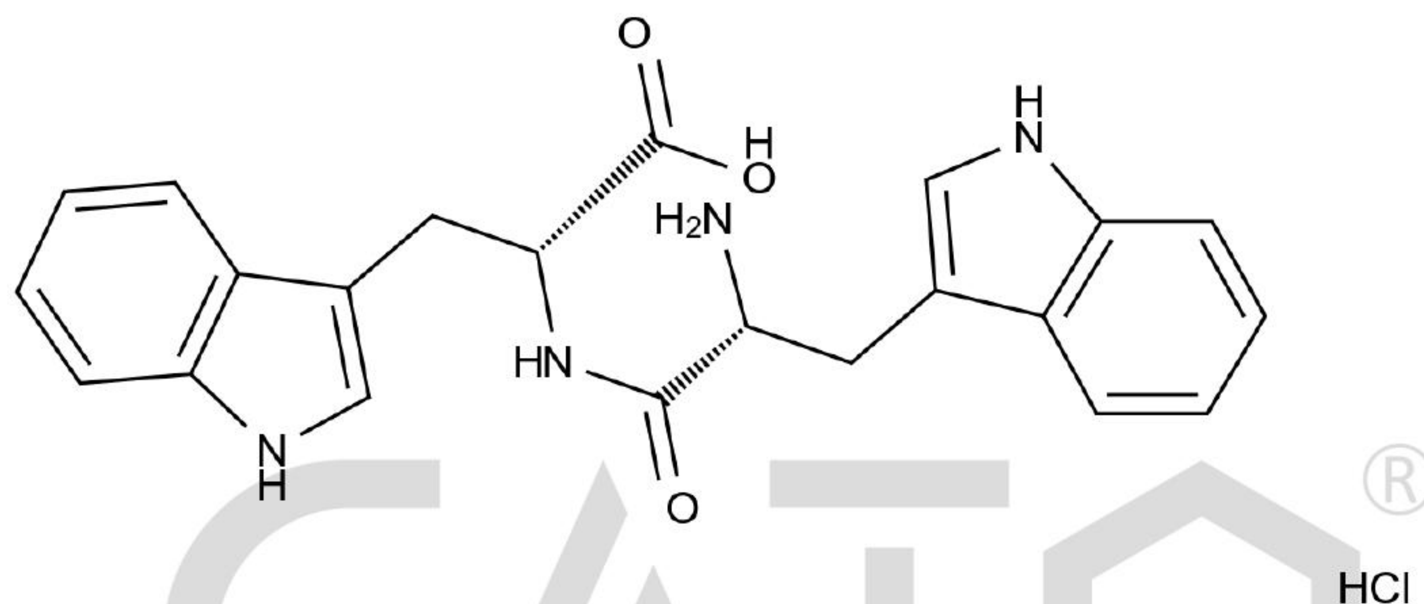
Chemical Structure:
