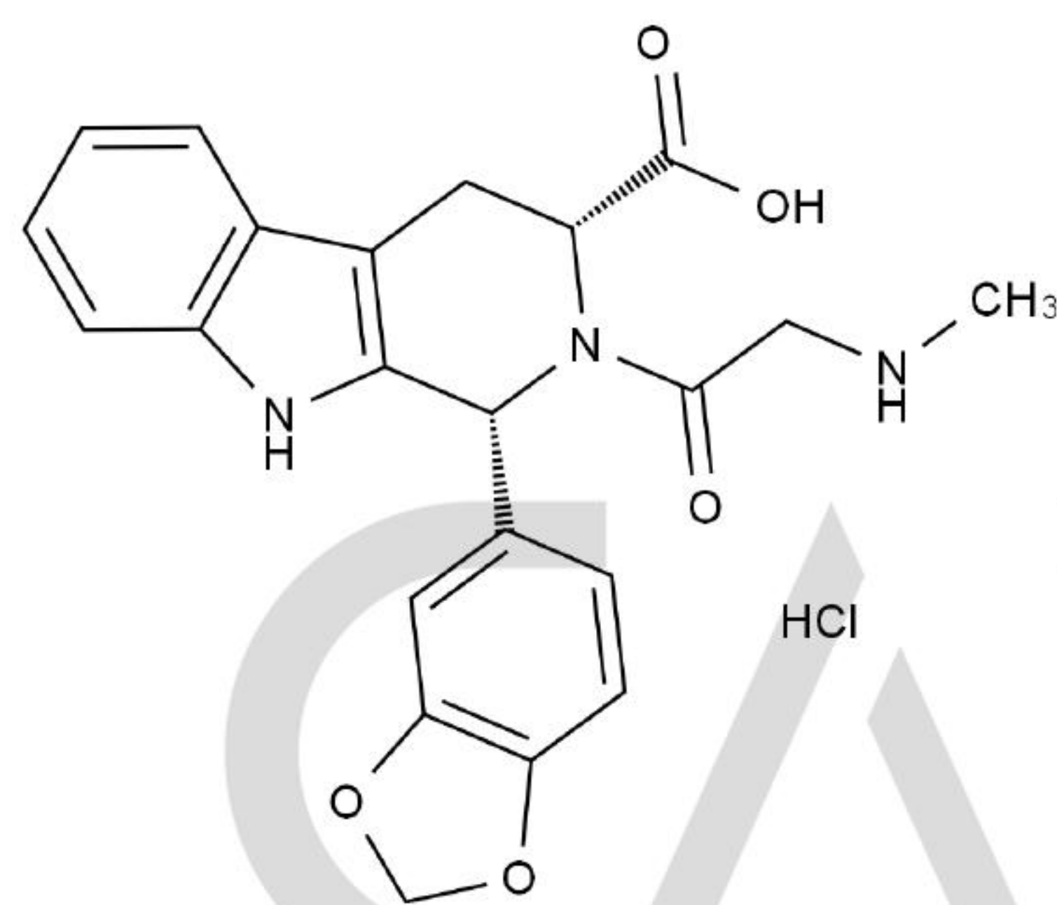
Chemical Structure:
