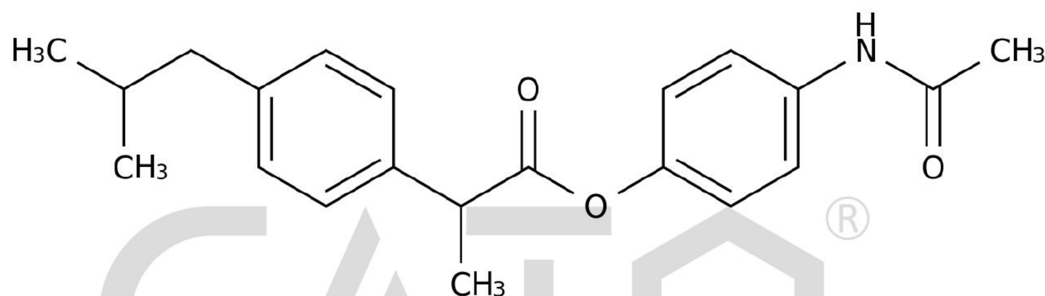
Chemical Structure:
