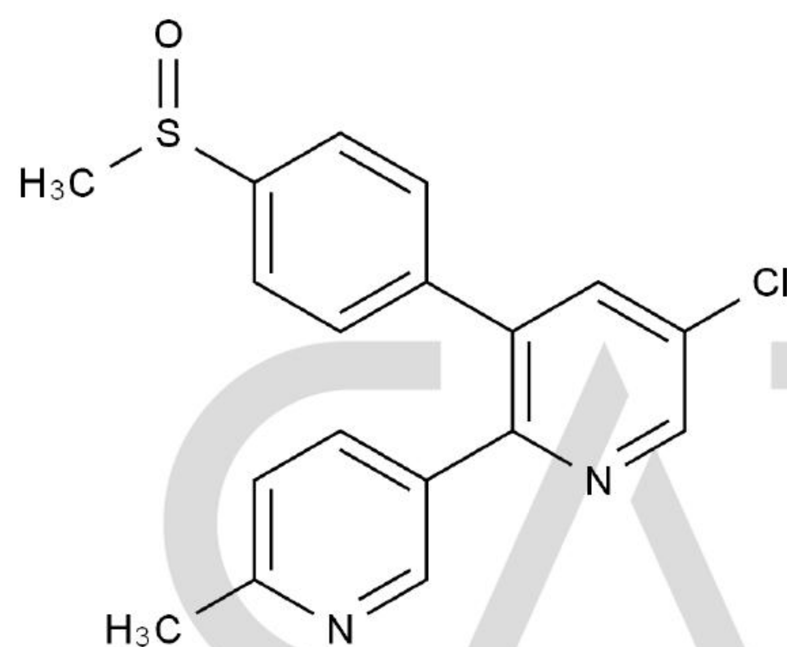
Chemical Structure:
