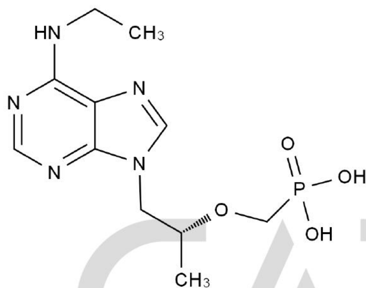
Chemical Structure:
