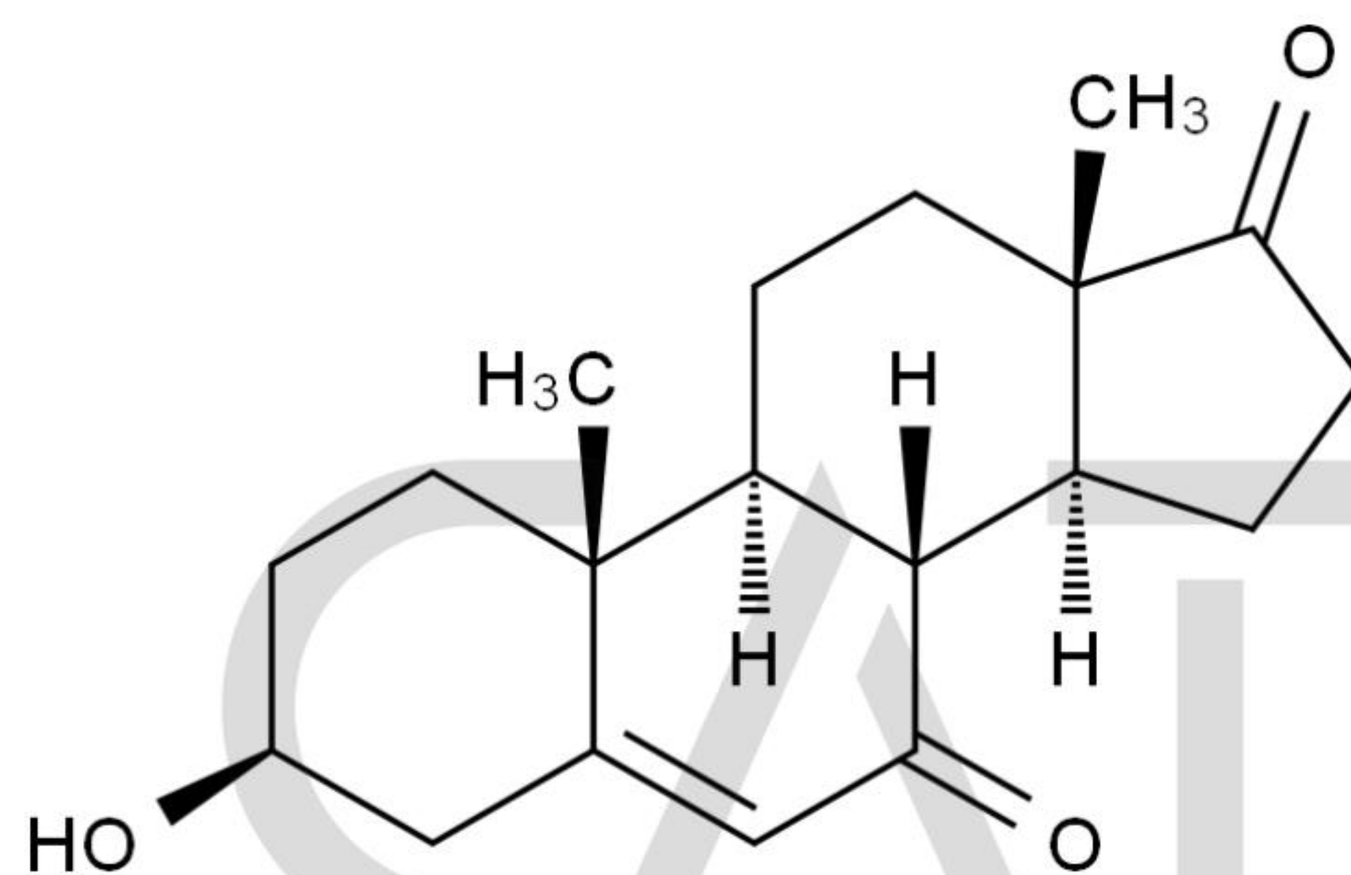
Chemical Structure:
