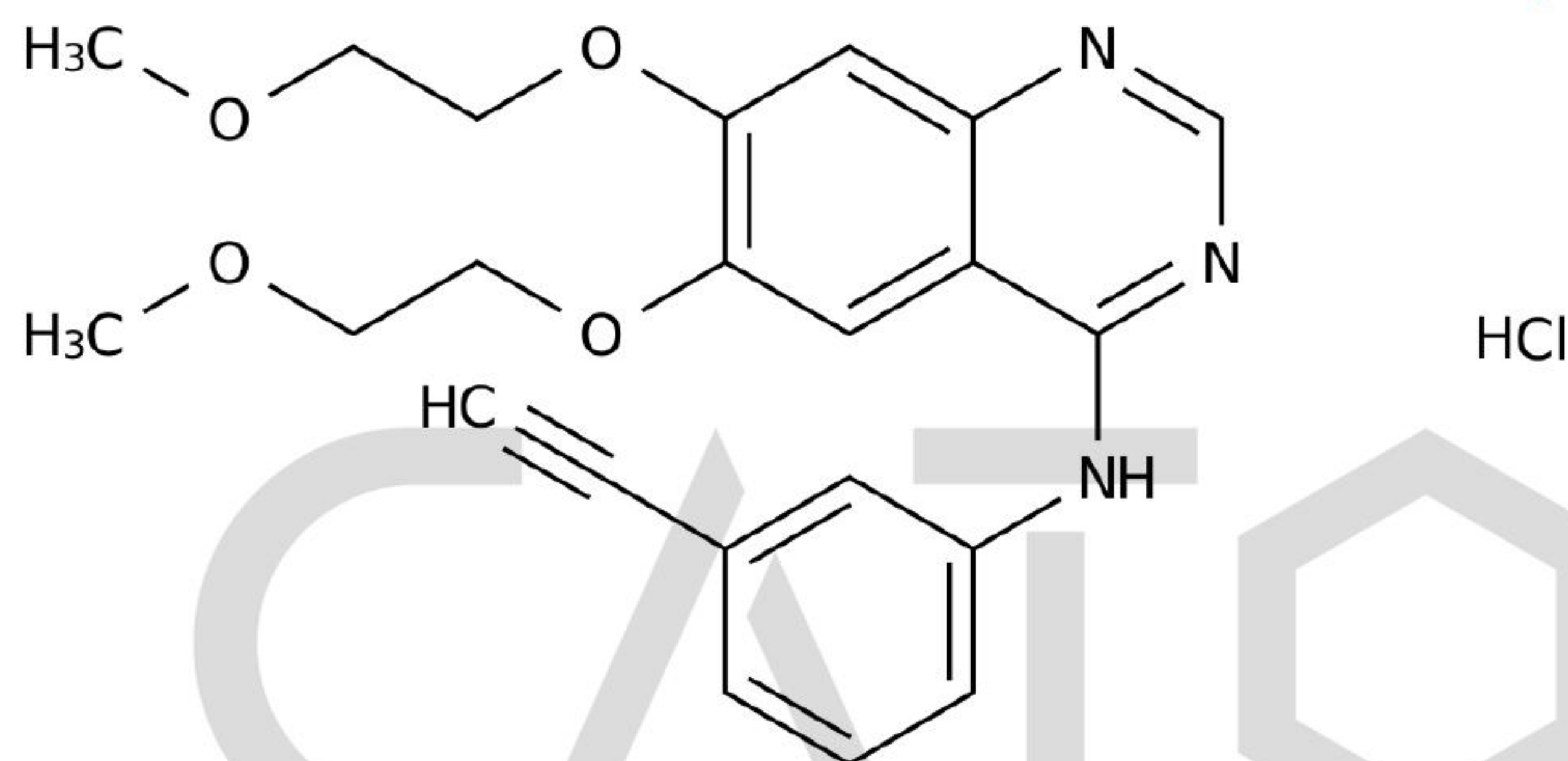
Chemical Structure:
