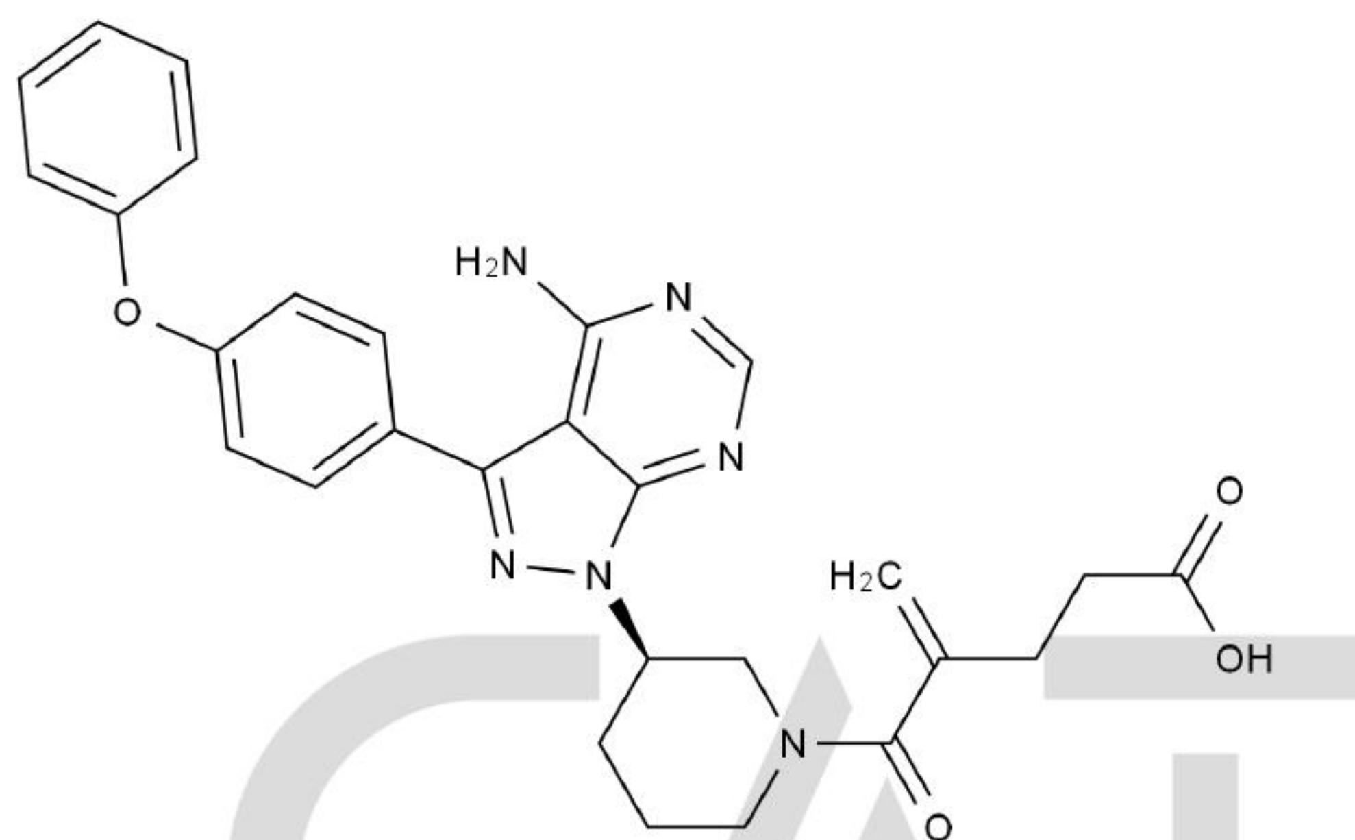
Chemical Structure:
