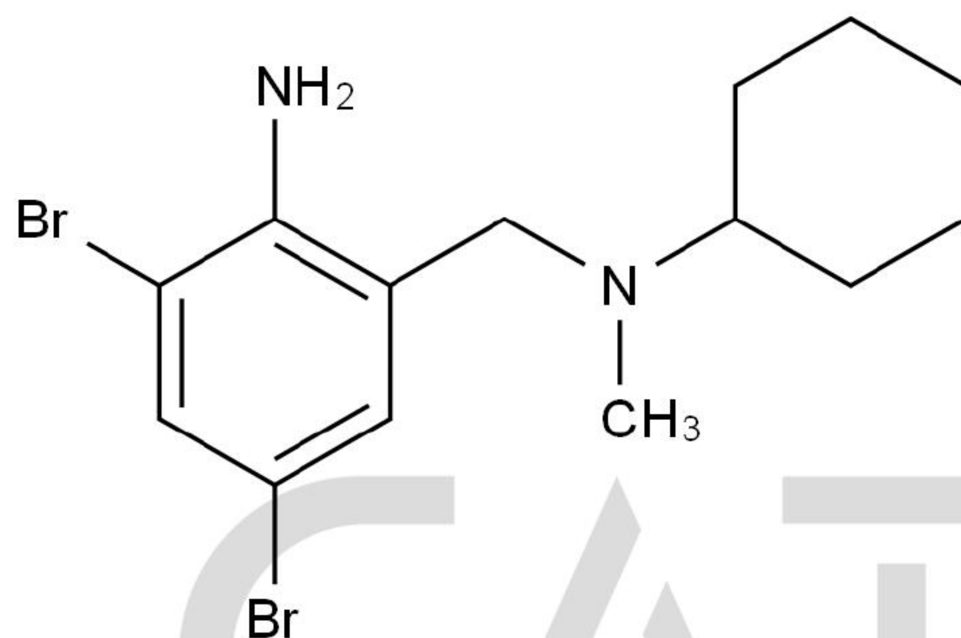
Chemical Structure:
