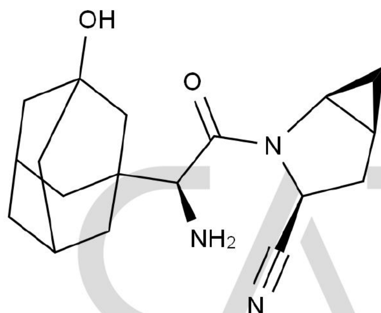
Chemical Structure:
