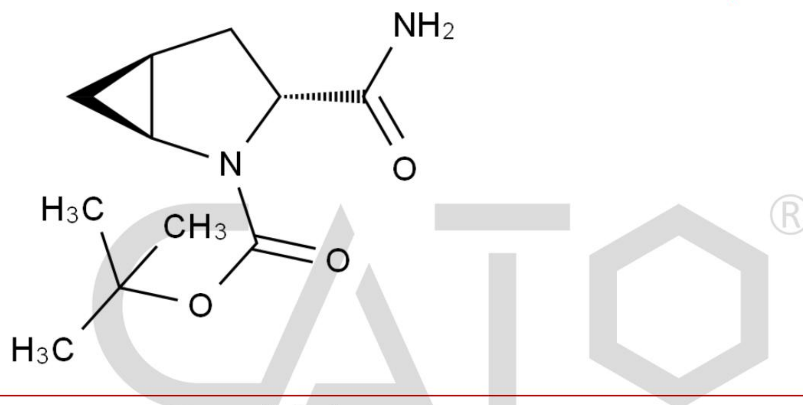
Chemical Structure:
