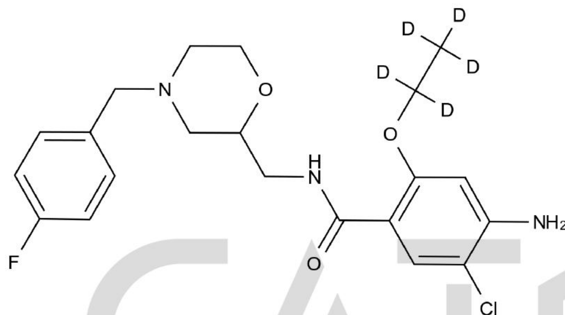
Chemical Structure:
