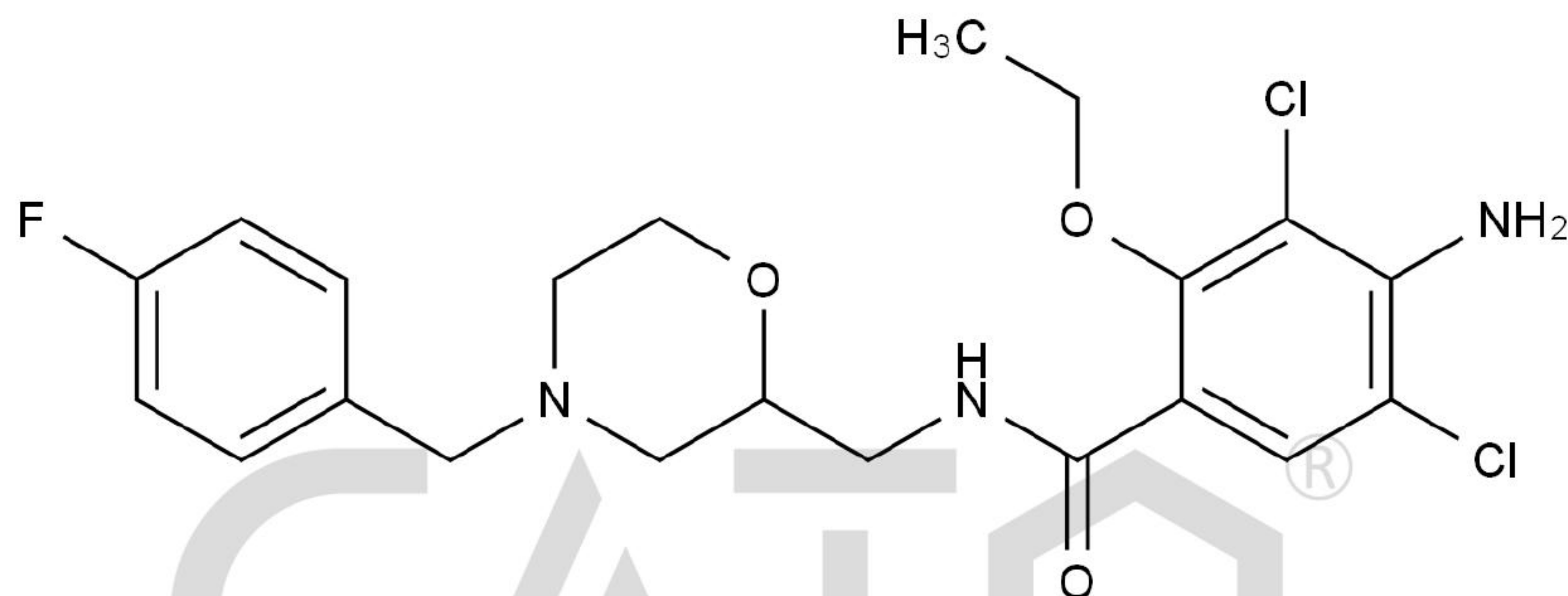
Chemical Structure:
