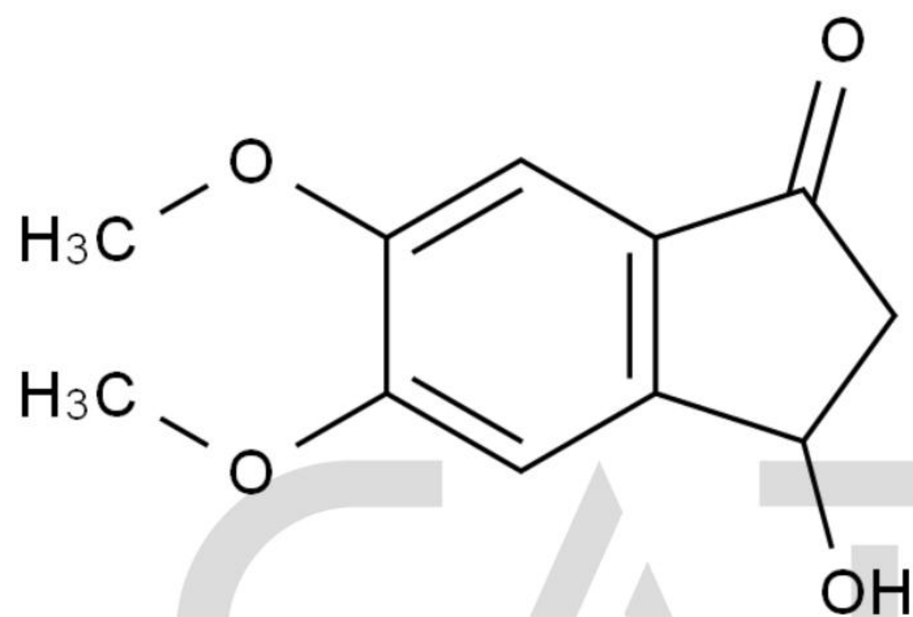
Chemical Structure:
