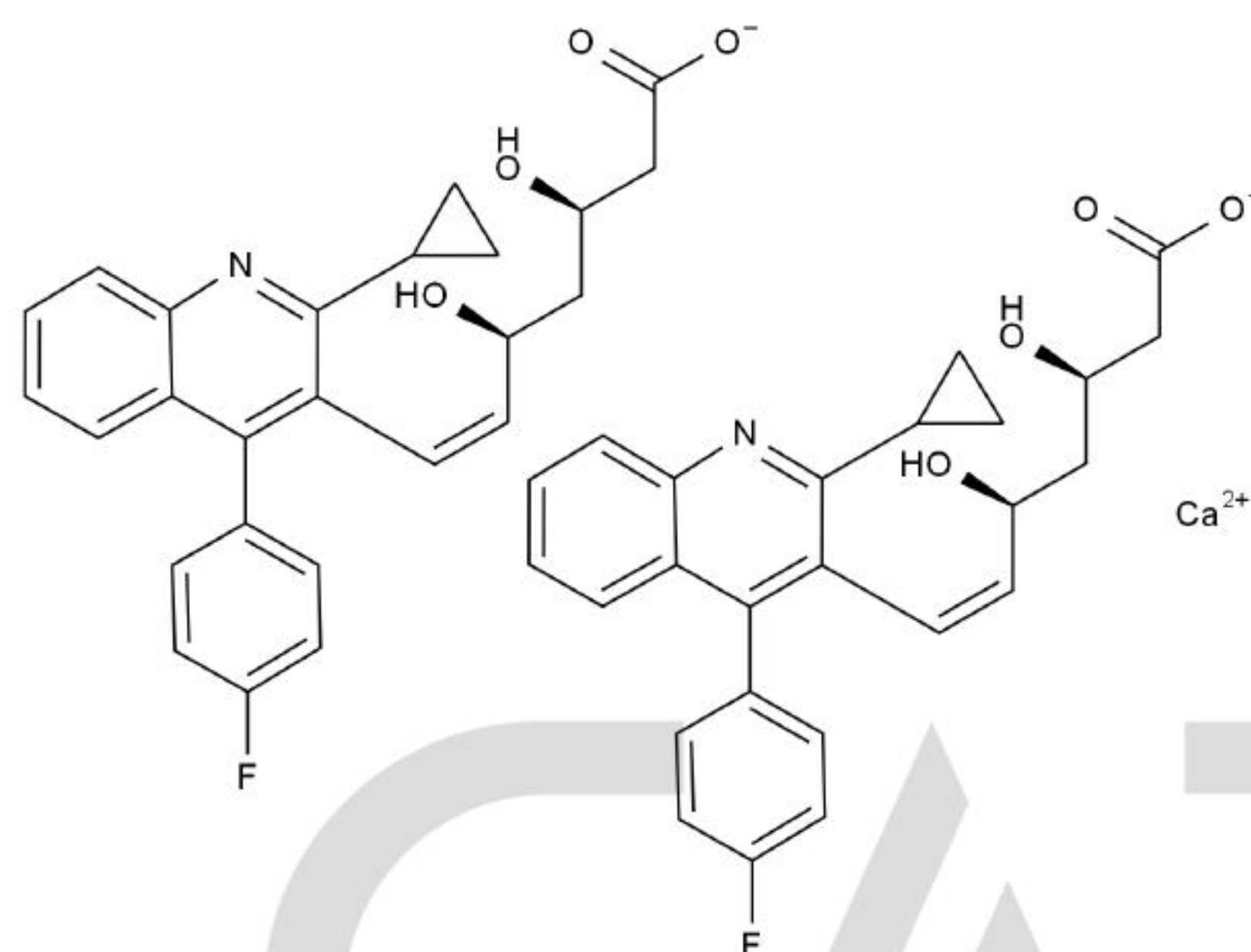
Chemical Structure:
