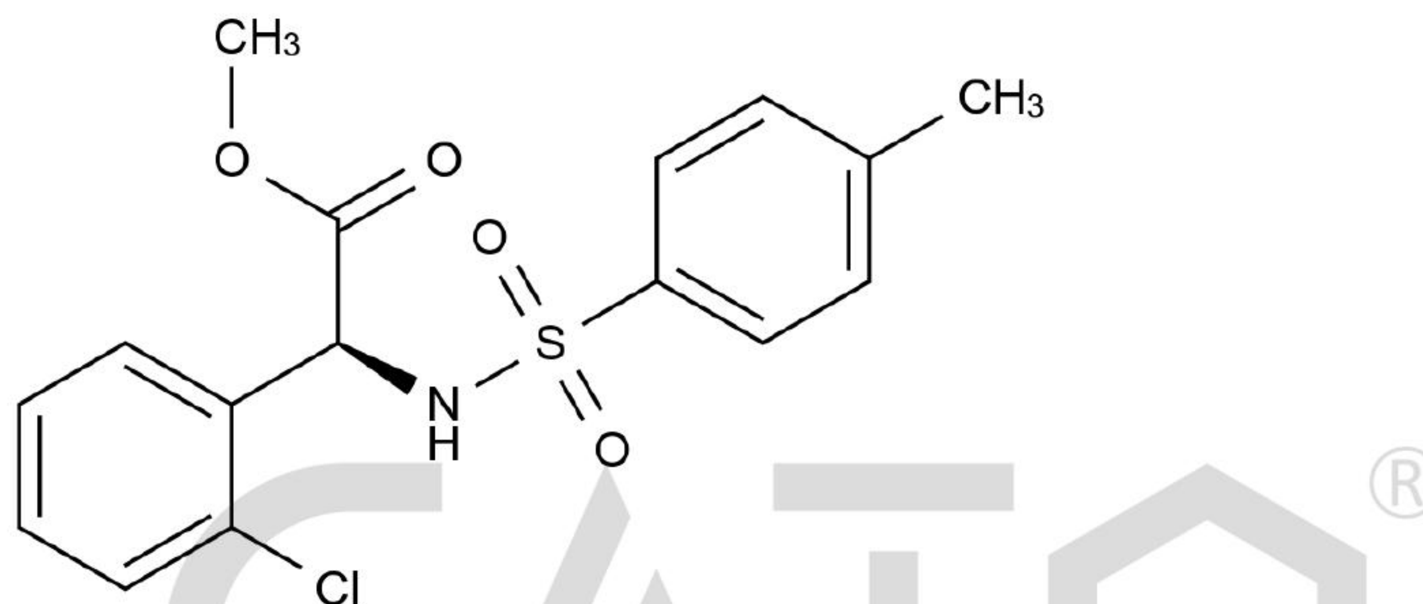
Chemical Structure:
