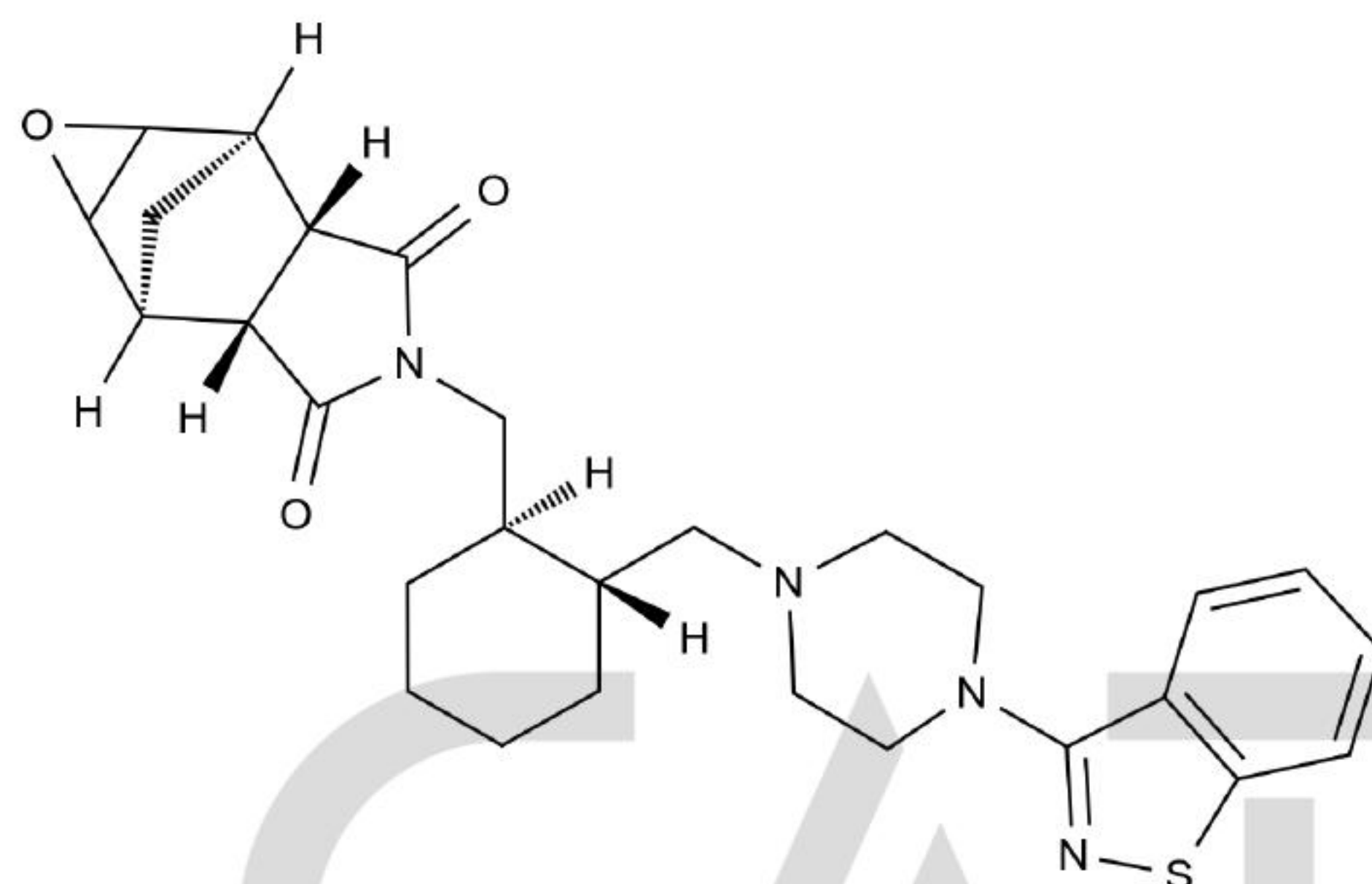
Chemical Structure:
