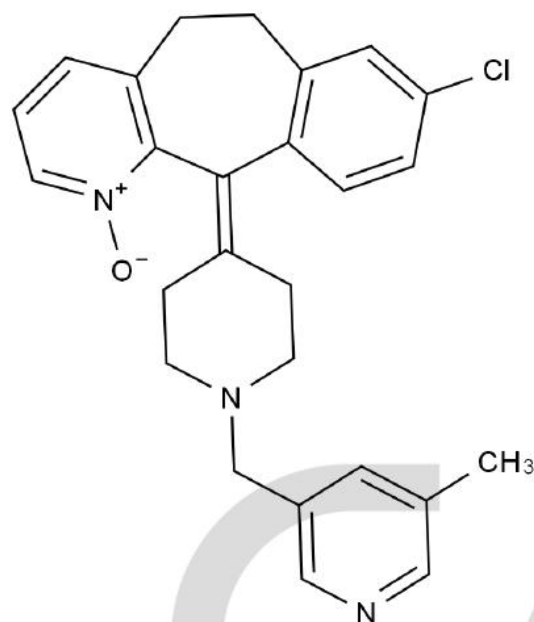
Chemical Structure:
