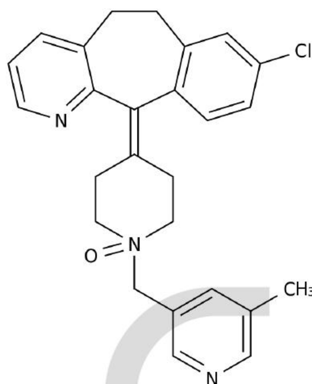
Chemical Structure:
